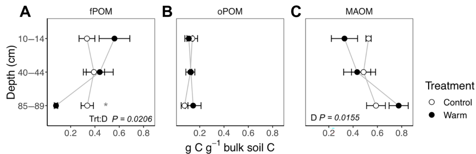
Fig. 2. Distribution of soil carbon among soil organic matter fractions. (A) fPOM, (B) oPOM, and (C) MAOM, (mean \pm SE, n = 3 ) sampled in June 2017, 3.5 years after the onset of warming. P are for any significant effects of treatment, depth, and their interaction (Trt:D). The asterisk indicates a significant treatment effect ( P_{1,2} = 0.02 ) at 85 to 89 cm in the fPOM fraction after within-depth, post hoc analysis. Stocks of carbon in each fraction are shown in fig. S3.
