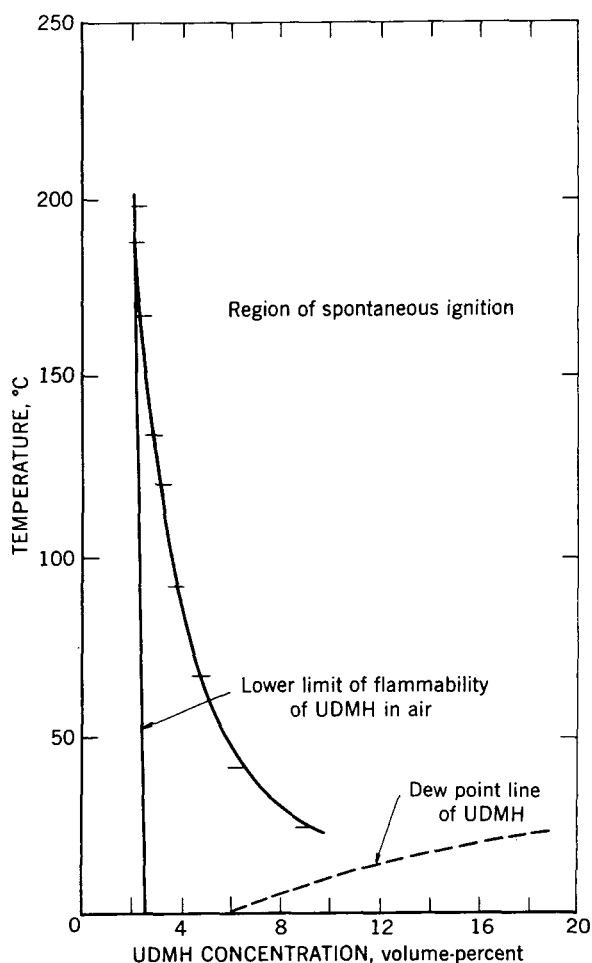
FIGURE 106.—Minimum Spontaneous Ignition Temperatures of Vaporized UDMH-Air Mixtures in Contact With 100 pct NO 2 at 25° C and 740 ± 10 mm Hg as a Function of UDMH Concentration in Air.
