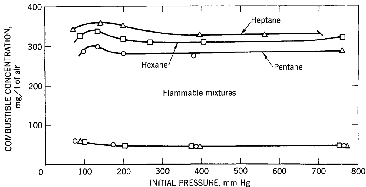
FIGURE 25.—Effect of Pressure on Limits of Flammability of Pentane, Hexane, and Heptane in Air at 26^\circ\text{C} .
