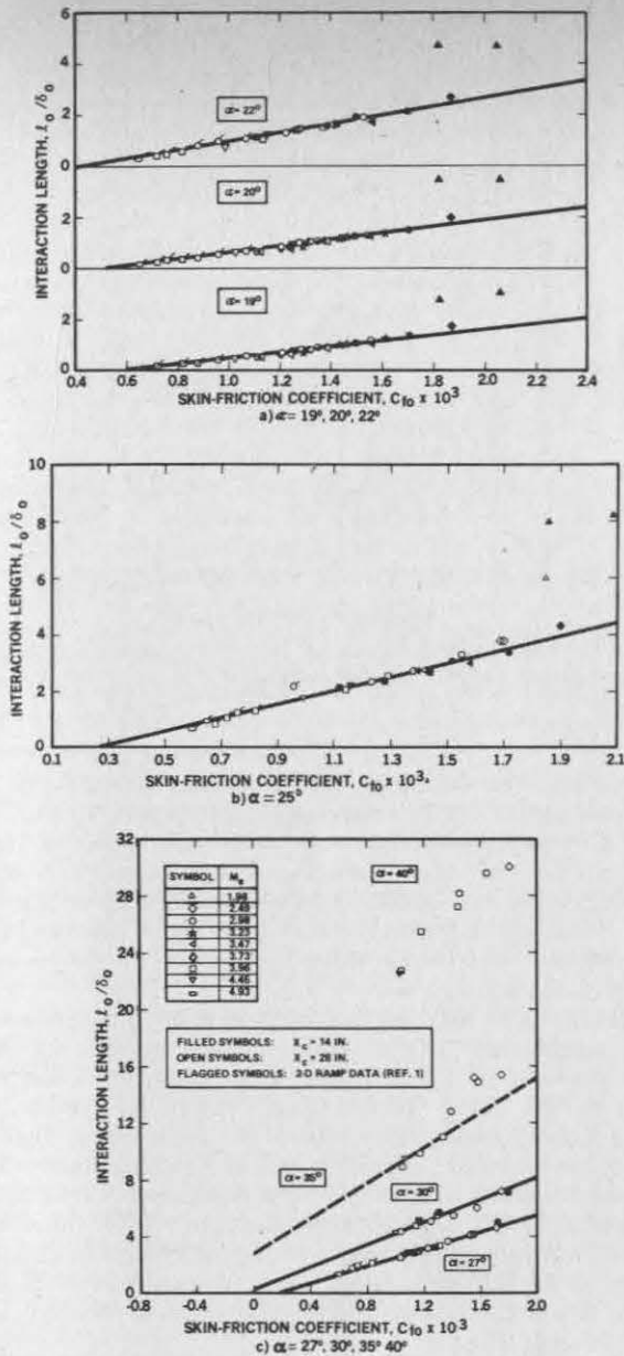
Fig. 8 Correlation of interaction length with local skin-friction coefficient: a) \alpha = 19^\circ, 20^\circ, 22^\circ ; b) \alpha = 25^\circ ; c) \alpha = 27^\circ, 30^\circ, 35^\circ, 35^\circ, 40^\circ .
