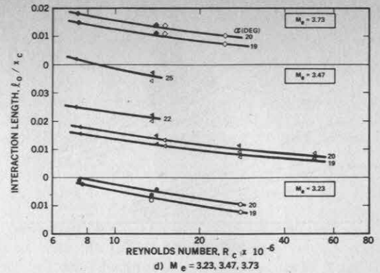
d) M_e = 3.23, 3.47, 3.73
