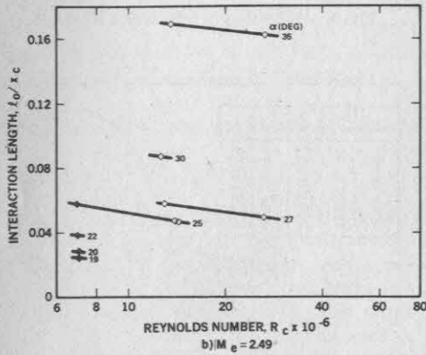
b) M_e = 2.49
