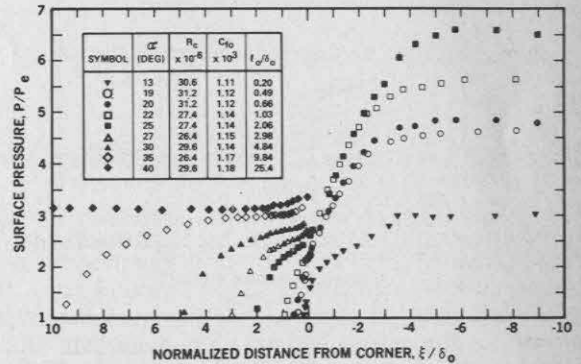
Fig. 5 Surface pressure distributions, M_e = 3.96 , x_c = 28 in.
