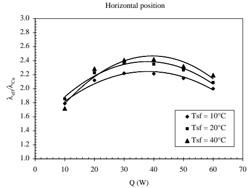
Fig. 11. Effective thermal conductivity enhancement variations Vs. Q, for different heat sink temperatures (Horizontal position)
