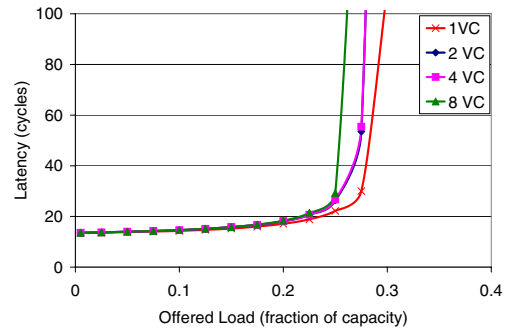
Figure 15. Performance comparison as the number of virtual channels is increased in the flattened butterfly.
