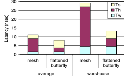
Figure 2. Latency of a packet in on-chip networks.
