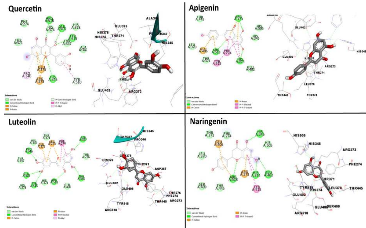
Fig. 5 Binding affinity of elected flavonoids to ACE-2 receptor
