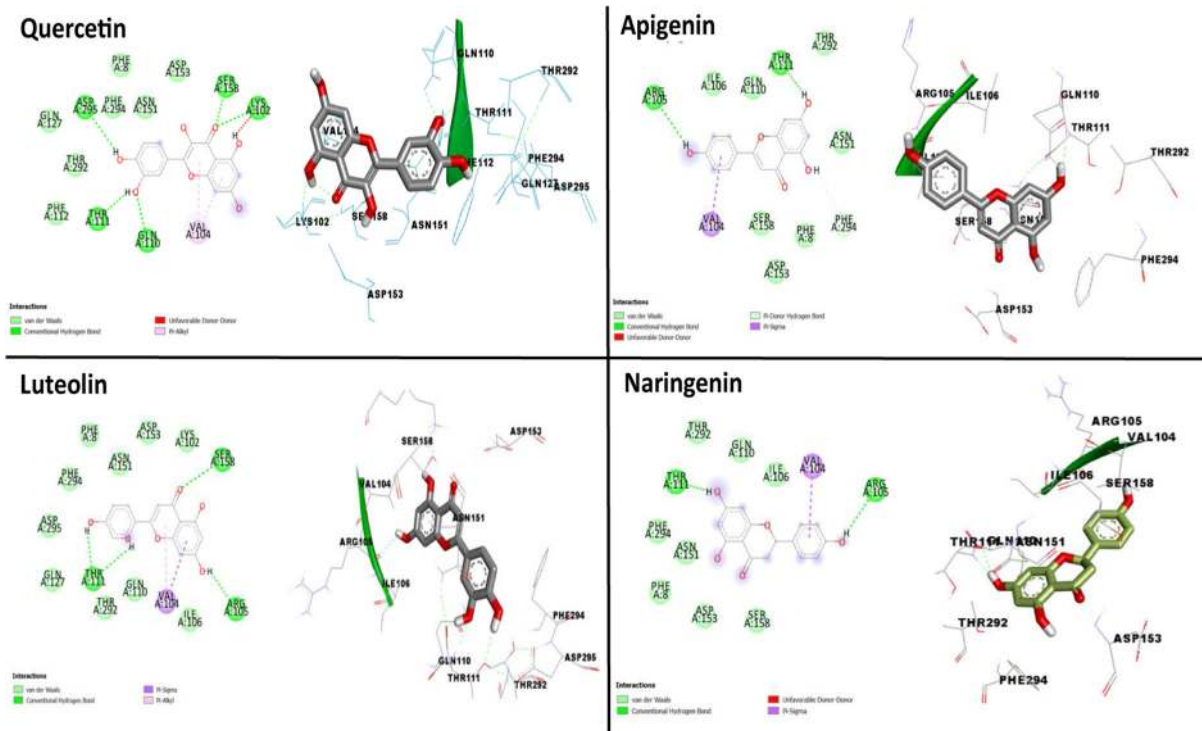
Fig. 4 Binding affinity of flavonoids to M PRO
