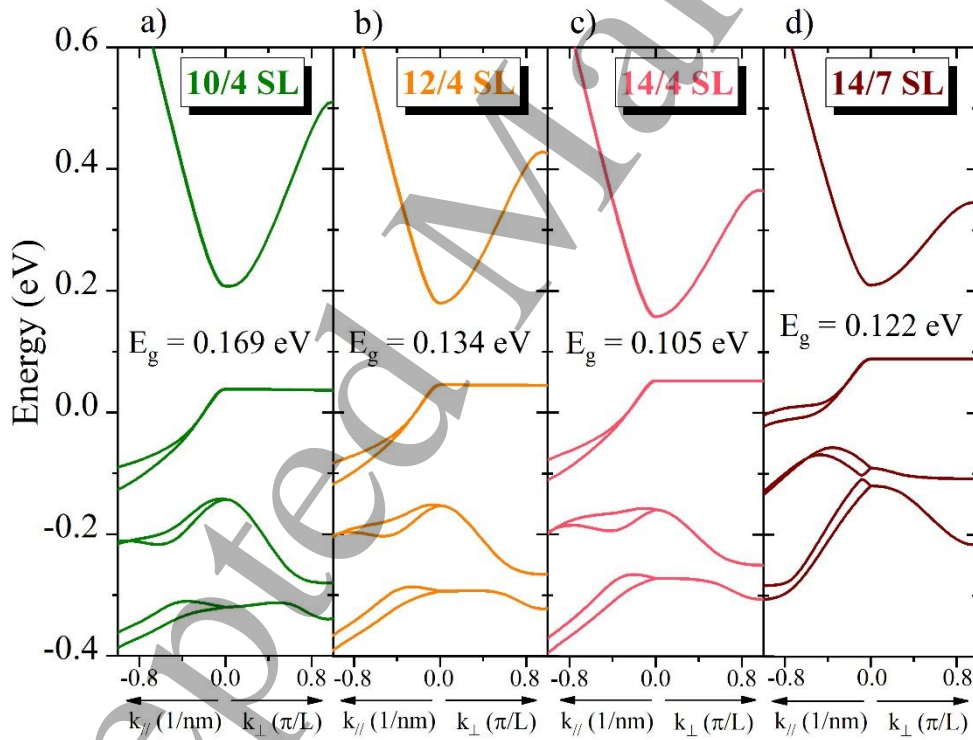
Figure 4: Calculated electronic band structure at 77K of (a) 10/4 SL, (b) 12/4 SL, (c) 14/4 SL and (d) 14/7 SL for the in-plane direction along [100] in the Brillouin zone k_{//} and in the perpendicular direction k_{\perp} (in units of \pi/L with L the period thickness).
