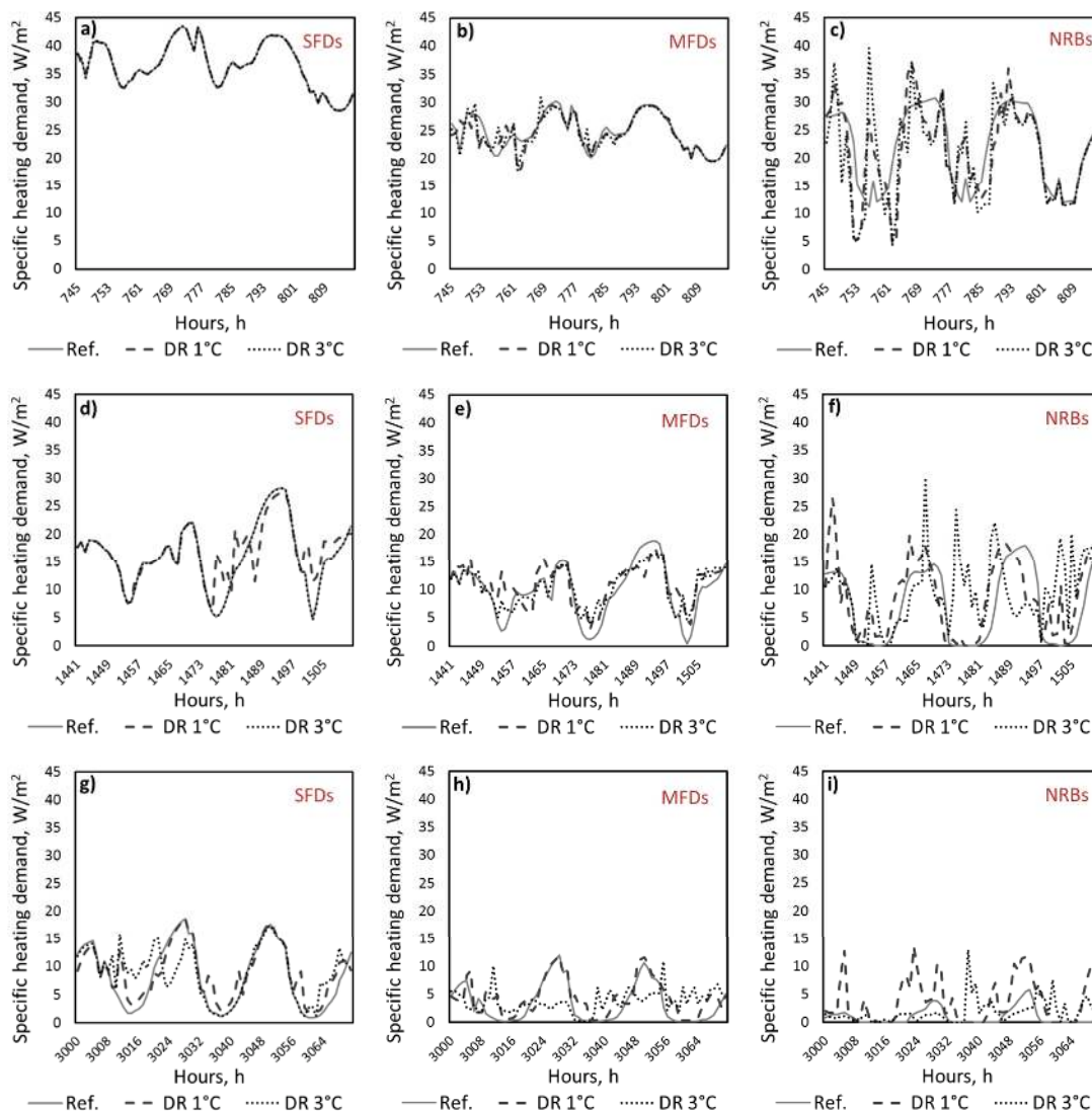
Figure 6. Specific ( W/m^2 ) hourly heating demand profiles of the SFDs, MFDs, and NRBs connected to the DH system of the City of Gothenburg, as obtained from the modeling for the Reference, DR 1 °C, and DR 3 °C scenarios. The profiles are shown for 3 days in: February, with average outdoor temperature of -10.7\text{ }^\circ\text{C} (a–c); March, with average outdoor temperature of 3.8\text{ }^\circ\text{C} (d–f); and May, with average outdoor temperature of 7\text{ }^\circ\text{C} (g–i), all in 2012.
