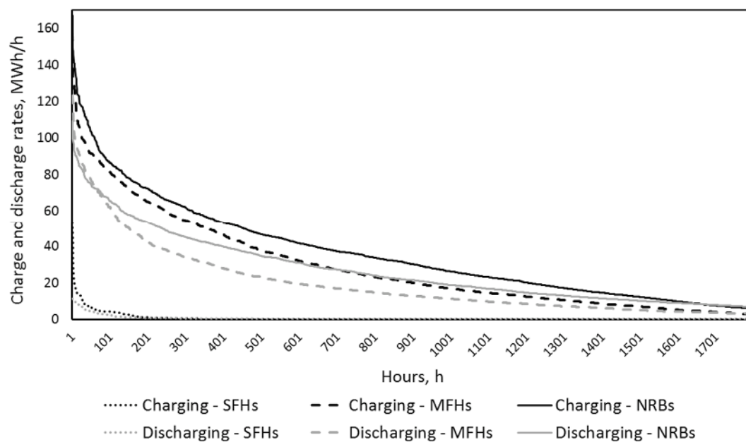
Figure 5. Duration curves for the hourly charging and discharging rates obtained from the modeling of the SFDs, MFDs, and NRBs connected to the DH system of the City of Gothenburg, for the Reference and DR 3 °C scenarios. Note that the x-axis only extends to 1800 h (during the remaining hours, the values are low, and thus, are not shown).
