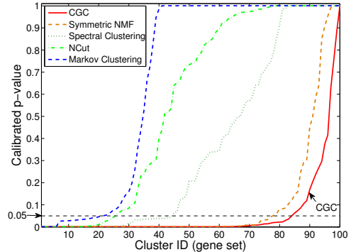
Figure 9: Comparison of CGC and single-domain graph clustering ( k = 100 )
