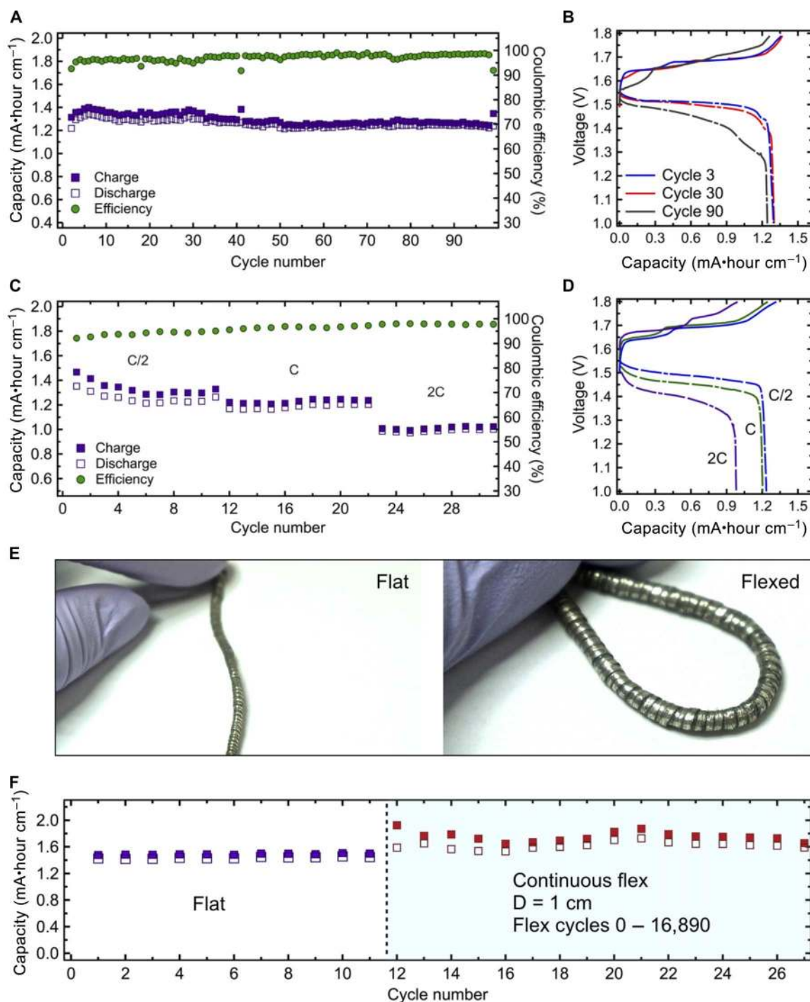
Fig. 2. Electrochemical and mechanical characterization of the flexible wire battery. (A) Capacity per unit length ( \text{mA}\cdot\text{hour cm}^{-1} ) and coulombic efficiency (%) of silver-zinc wire battery cycled at 0.25C charge and 0.5C discharge rates between 1 and 1.8 V. (B) Galvanostatic charge-discharge curves for cycles 3, 30, and 90 of the battery in (A). (C) Specific capacity ( \text{mA}\cdot\text{hour cm}^{-1} ) and coulombic efficiency (%) of silver-zinc wire battery cycled between 1 and 1.8 V at charge rates C, 0.5C, and 0.25C and discharge rates 2C, C, and 0.5C, respectively. (D) Galvanostatic charge-discharge curves of the battery in (C). (E) Optical images of the flexible wire battery in a relaxed and deformed state. (F) Cycling performance of the battery operated in a flat configuration and while being continuously flexed to a bending diameter ( D ) of 1 cm.
