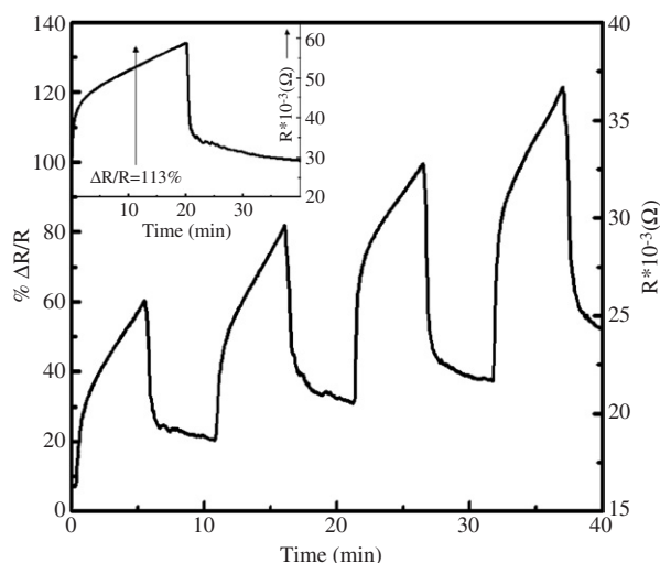
Figure 6. Sensor response of SWNT/PET device to DMMP saturated vapour (1620 ppm at 21°C) under ambient laboratory conditions. Exposure and evacuation cycles 5 min. Inset: exposure and evacuation cycles 20 min.
