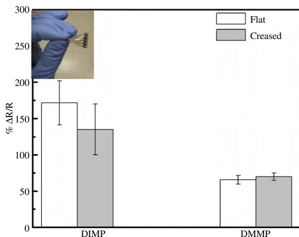
Figure 4. Sensor response of flat (bending angle 180°) and creased (clasped with a paper clip with a bending angle ~5°) SWNT/PET device when exposed to simulant vapours at saturated vapour concentrations. Inset: optical image of sensor when bent to a crease.
