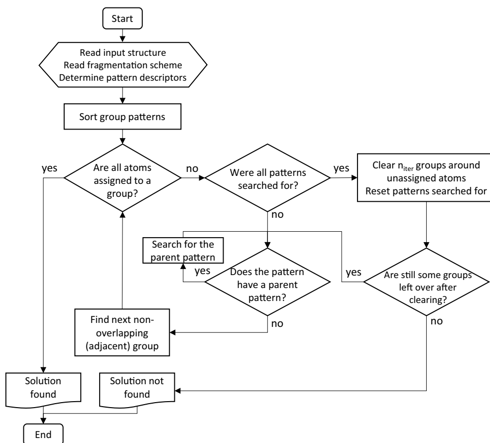
Fig. 3 Schematic representation of the simple fragmentation algorithm
