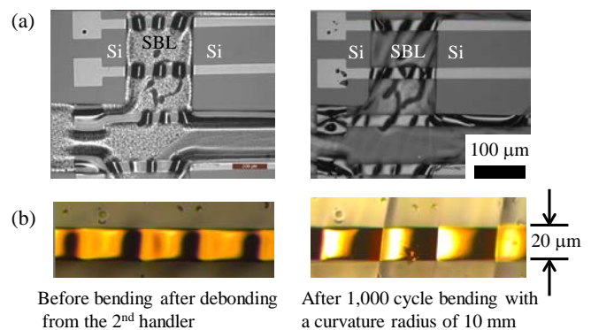
Fig. 14. SEM images (a) and the enlarged photomicrographs (b) of 600-nm-thick Cu wirings formed on FlexTrate™ with dielets embedded in PDMS before and after bending.
