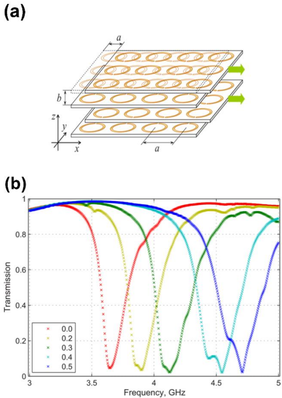
FIG. 11. Lattice displacement to create a reconfigurable metamaterial. (a) Schematic representation of shifting metasurfaces in relation to other layers. (b) Transmission response of the waveguide with different metamaterial slabs. Graphs with dips from right to left correspond to decreasing lattice shift. Image reproduced with permission from Appl. Phys. Lett. 95, 084105 (2009). Copyright 2009 American Institute of Physics
