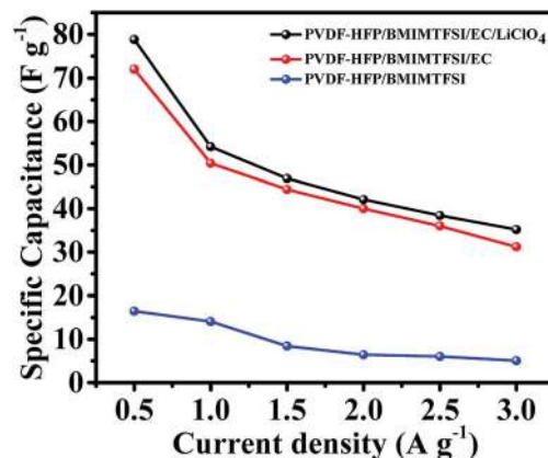
Fig. 7 Capacitance curves of the symmetric supercapacitors with the PVDF-HFP/BMIMTFSI electrolyte, the PVDF-HFP/BMIMTFSI/EC electrolyte, and the PVDF-HFP/BMIMTFSI/EC/LiClO 4 electrolyte with current densities from 0.5 to 3 A g -1 .
