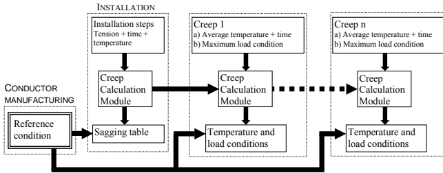
Fig. 13. Schematic diagram of STOC.
