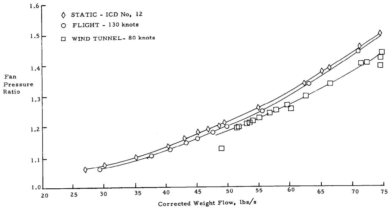
Figure 40.- Fan operation comparisons for JT15D with hardwall inlet.
