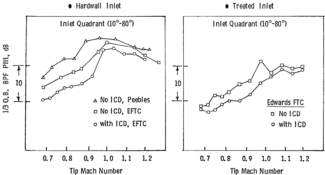
Figure 34.- CF6-80A ICD test results.
