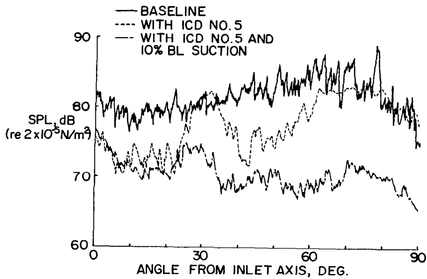
Figure 68.- JT15D fan boom microphone blade passage tone directivity; 10,500 corrected rpm.
