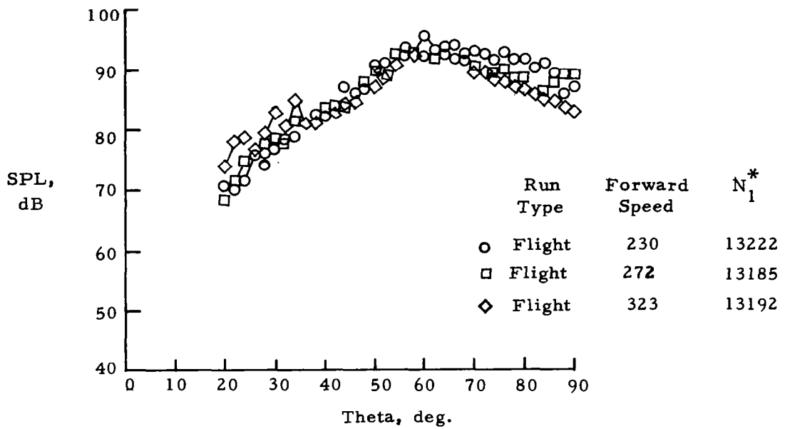
Figure 147.- Forward speed effects on BPF noise.
