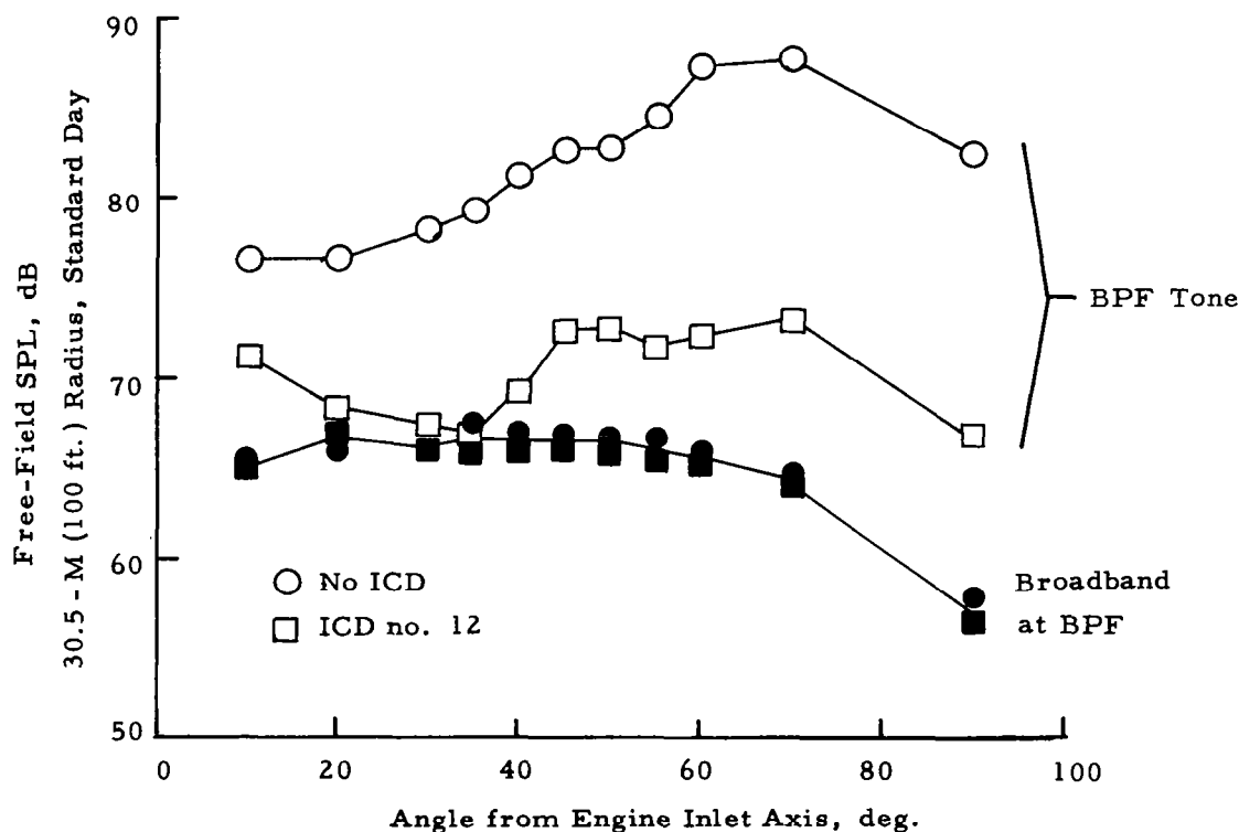
Figure 44.- BPF directivity with "flight" inlet; NF = 10,800 rpm.
