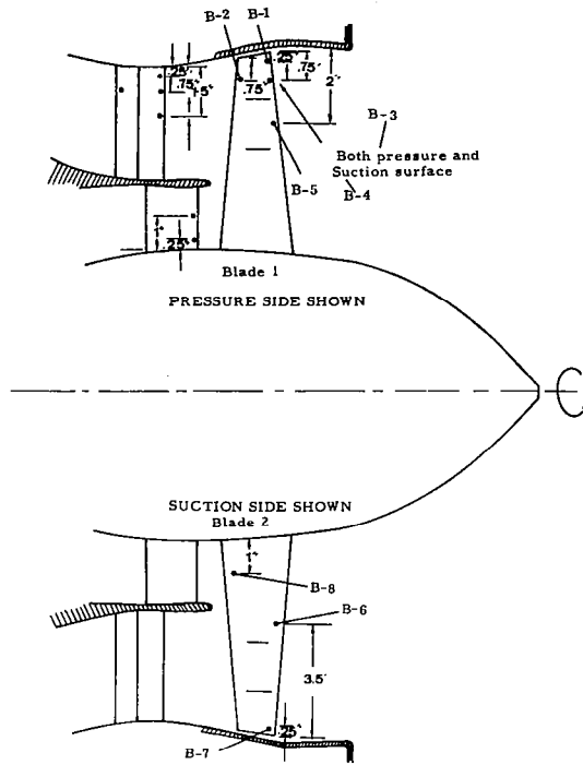
Figure 37.- JT15D-1 transducer locations and designations.
