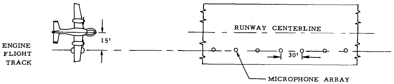
Figure 127.- Plan view of flight profile.
