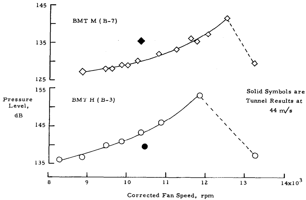
Figure 139.- Amplitude of 6th harmonic of fan speed in flight.
