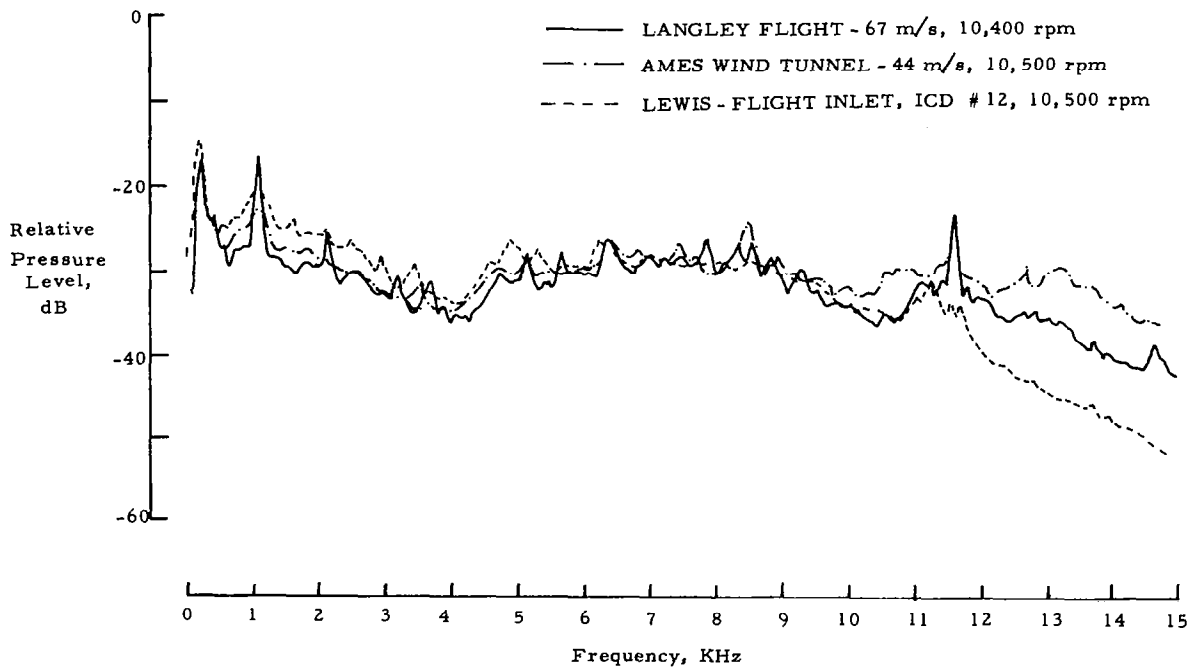
Figure 140.- Overall spectra, BMT H (Lewis B-3), for flight, tunnel, and static.
