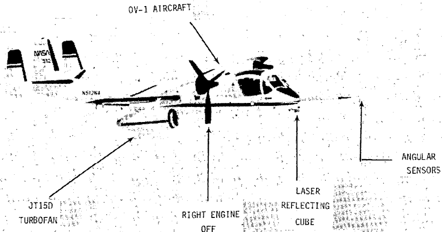
Figure 123.- Test aircraft.
