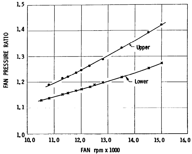
Figure 94.- Two fan operating lines tested.
