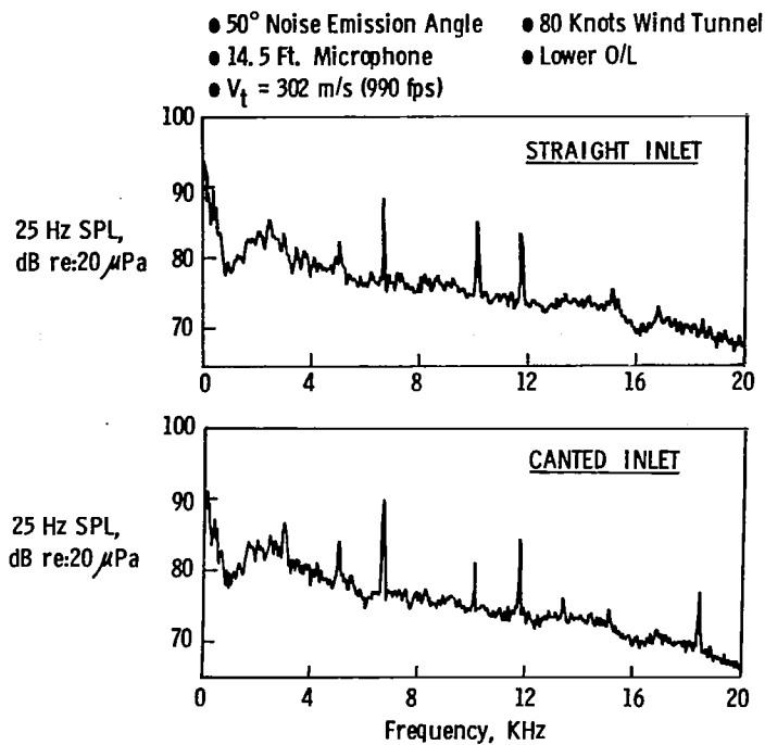
Figure 91.- Comparison of canted and straight diffusing with treated inlet - narrowband spectra.
