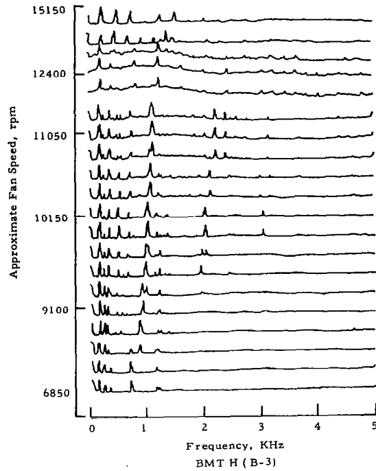
Figure 137.- BMT spectra from sweep of fan speed during flight; 67 m/s, BMT H (Lewis B-3).
