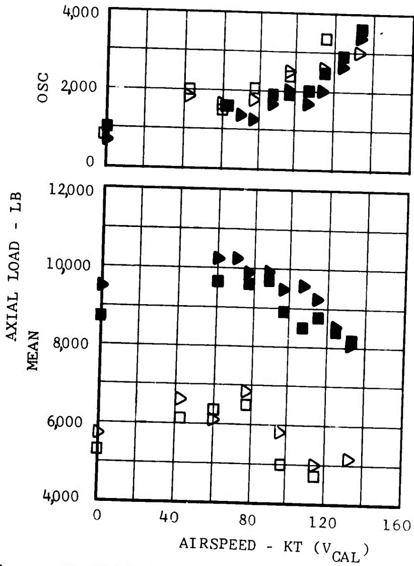
Figure 35. Main Rotor Red Drag Brace Loads Versus Airspeed.
