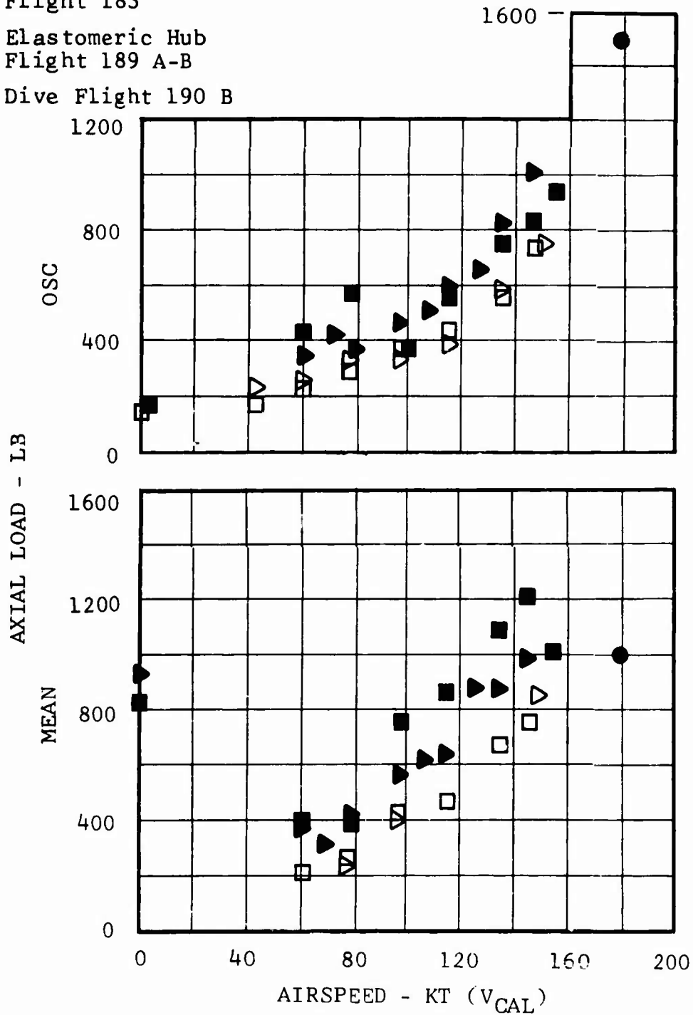
Figure 25. Collective Boost Tube Loads Versus Airspeed.
