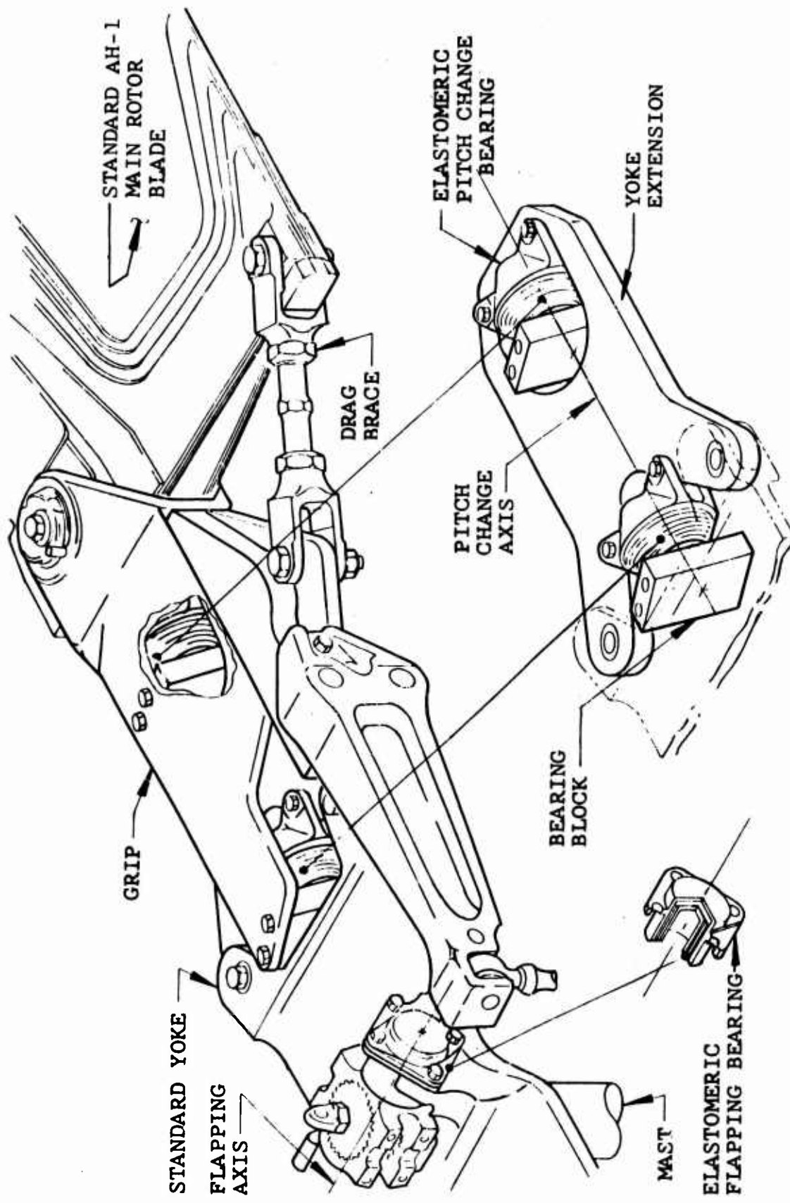
Figure 1. Elastomeric Bearing Rotor Hub.
