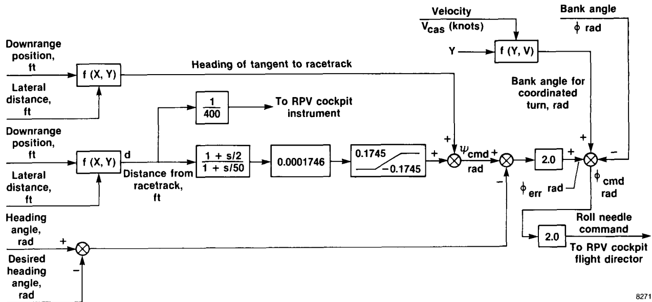
Figure 21. Lateral racetrack guidance control law.
