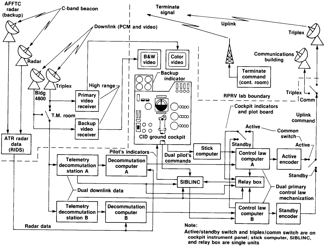
Figure 6. B-720 jet transport controlled impact demonstration ground remotely piloted vehicle control system.
