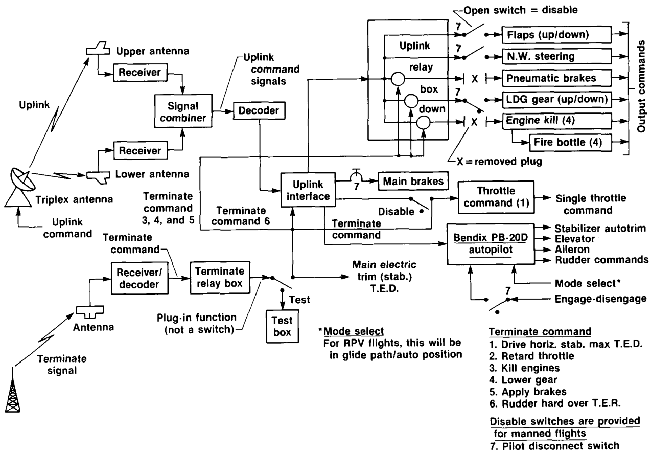
Figure 10. B-720 controlled impact demonstration airborne remotely piloted vehicle control system.
