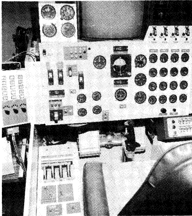
Figure 8. Remotely piloted vehicle ground cockpit.
