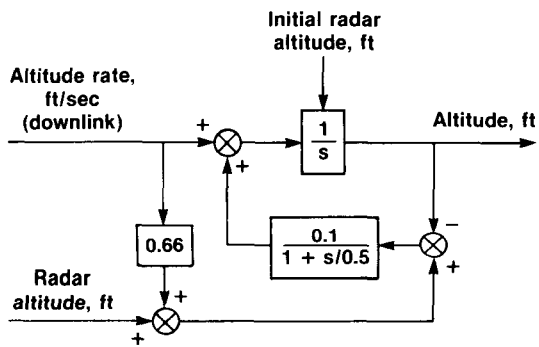
(c) Altitude calculation.
