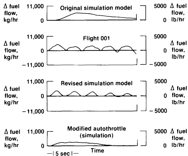
Figure 24. Comparison of flight and simulation engine fuel-flow response to an autothrottle step input.
