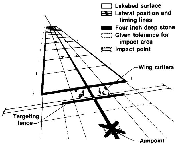
Figure 1. Controlled impact demonstration layout.
