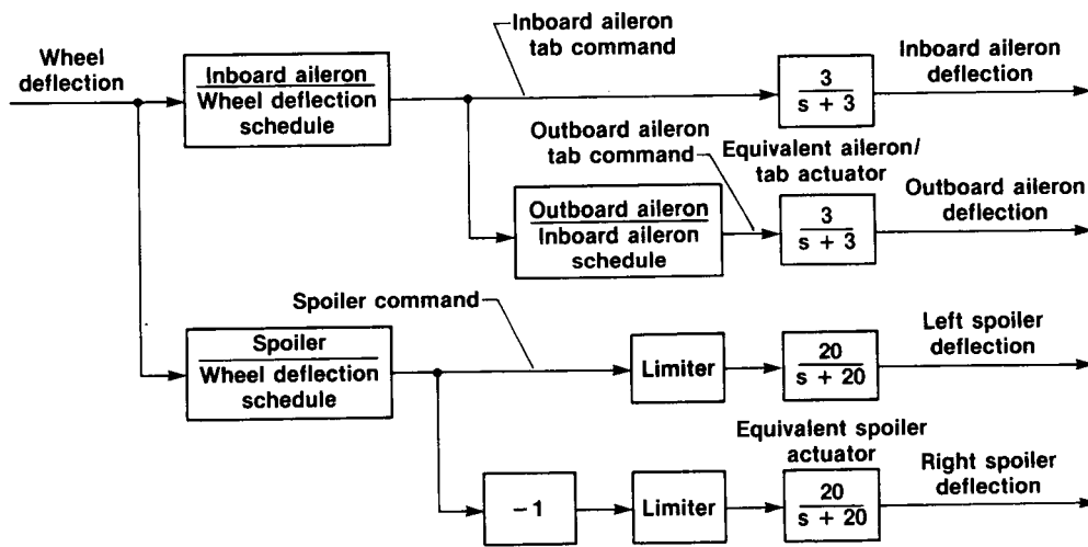
(b) Aileron and spoiler command path.
