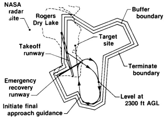
Figure 4. Controlled impact demonstration ground track and sterile area boundary.
