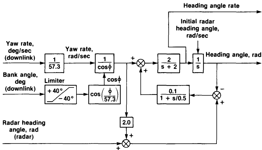
(a) Heading angle calculation.
