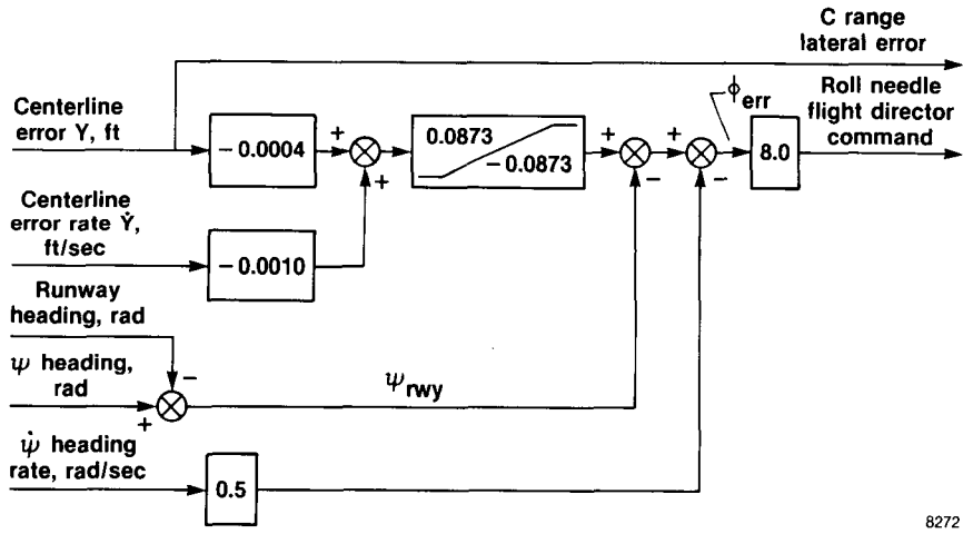
Figure 22. Lateral final approach control law.
