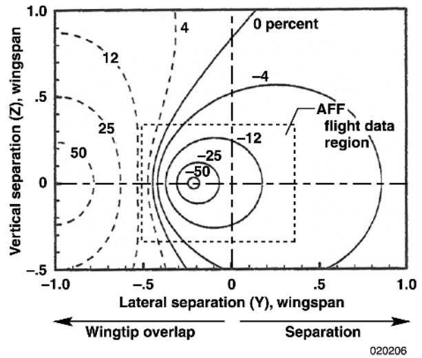
Figure 2. Predicted variation in mutual induced drag with aircraft position using the horseshoe vortex model.
