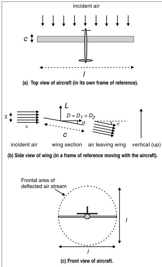
Fig. 1. Simple model of air flowing around a wing.
