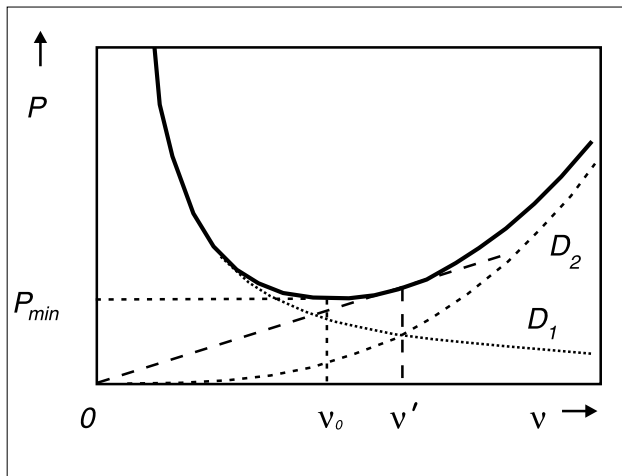
Fig. 2. Dependence of power on flight velocity for level flight without acceleration. The two velocities marked are those for minimum power ( v_0 ) and maximum range ( v' ). The two types of drag responsible for power consumption are induced drag ( D_1 ) and friction drag ( D_2 ).
