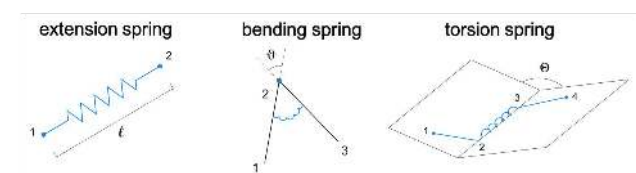
Figure 4: The three types of spring elements considered to model the arches in the stick-and-spring model, associated to edges, wedges, and z-edges.
