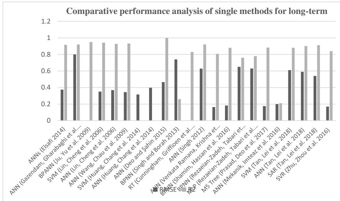
Figure 9. Comparative performance analysis of single methods of ML for long-term prediction.
