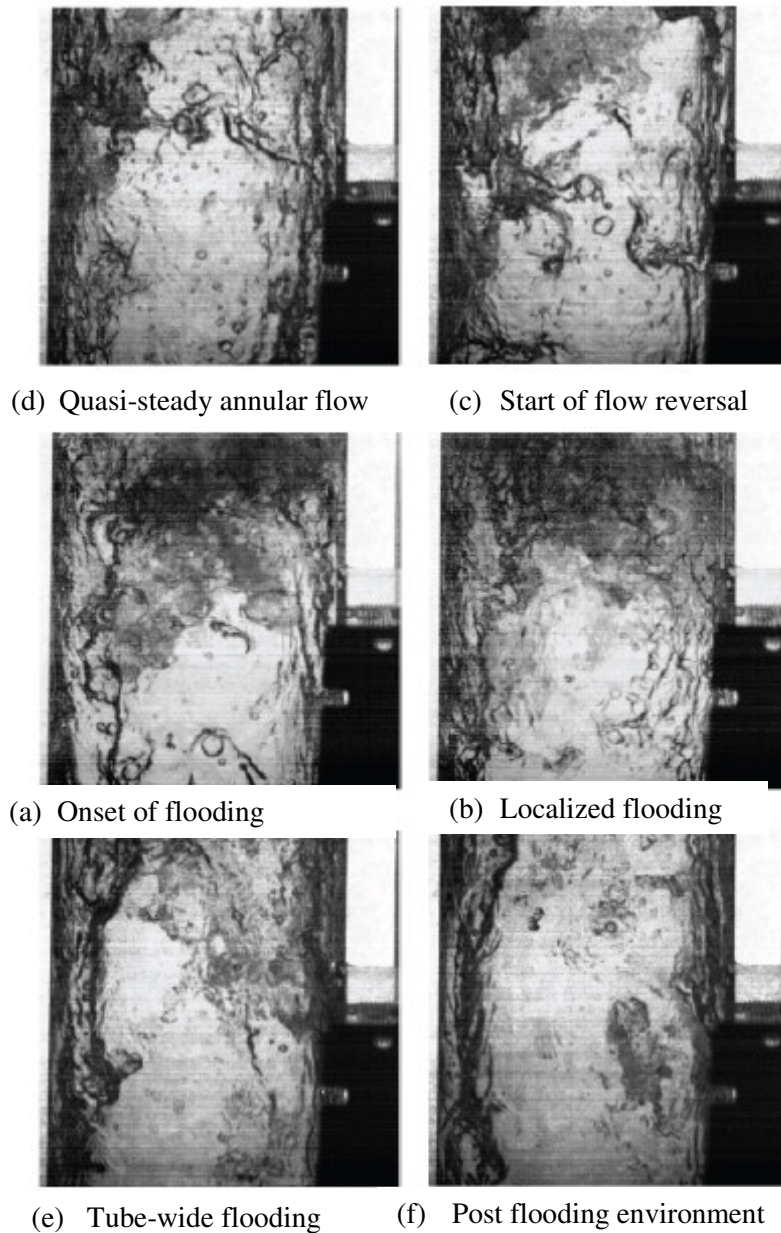
Figure 5 Flooding Visualization
