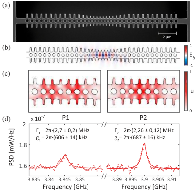
FIG. 2. (a) Scanning electron microscope image of the fabricated optomechanical cavity. (b) Simulated electric field pattern of the optical mode. The measured resonance wavelength is \lambda_r = (1527.4 \pm 0.2) nm with loaded decay rate \kappa/2\pi = (14.88 \pm 0.08) GHz. (c) Calculated mechanical displacement profiles of P1 and P2. (d) Measured power spectral density of the thermally transduced mechanical modes at \Omega_1/2\pi = 3.845 GHz and \Omega_2/2\pi = 3.899 GHz.
