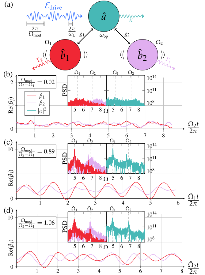
FIG. 1. (Color online) Multimode phonon lasing in an optomechanical cavity. (a) Two mechanical modes at distinct frequencies are coupled to an optical cavity driven by an intensity-modulated pump. (b) For small modulation frequency both mechanical modes remain in a thermal state. (c) With the modulation frequency approaching the difference frequency only one mode ( \beta_1 ) transitions into SSO with the help of the multimode gain mechanism, whereas the other mode remains in the thermal state while being driven at \tilde{\Omega}_1 + \Omega_{\text{mod}} . (d) When the modulation frequency approximates the difference frequency, both mechanical modes coherently oscillate, i.e., MMO occurs. Insets show the power spectral densities of the mechanical (left) and optical (right) modes.
