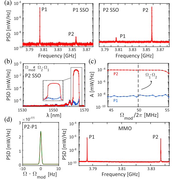
FIG. 3. From single-mode to multimode phonon lasing. (a) Self-oscillation spectra of P1 (left) and P2 (right), without external modulation. (b) P2 SSO excitation through a wavelength scan with a blue-detuned laser \Omega_{\text{mod}} \neq \Omega_2 - \Omega_1 . (c) Mechanical amplitude evolution in a modulation frequency scan around the difference frequency when P2 is self-oscillating showing that hysteretic effects prohibit the MMO state from being activated from the SSO state. (d) Multimode lasing under an input modulation \Omega_{\text{mod}} = \Omega_2 - \Omega_1 . Left: difference tone obtained by mixing the lasing mechanical modes in the microwave domain, proving mode locking. Right: spectrum of the two mechanical modes when lasing simultaneously (MMO state).
