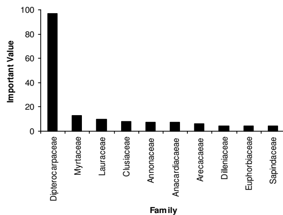
Figure 3. Ten most important families for sapling. Family Importance Value is sum of Importance Value of all species contained in a single family.
