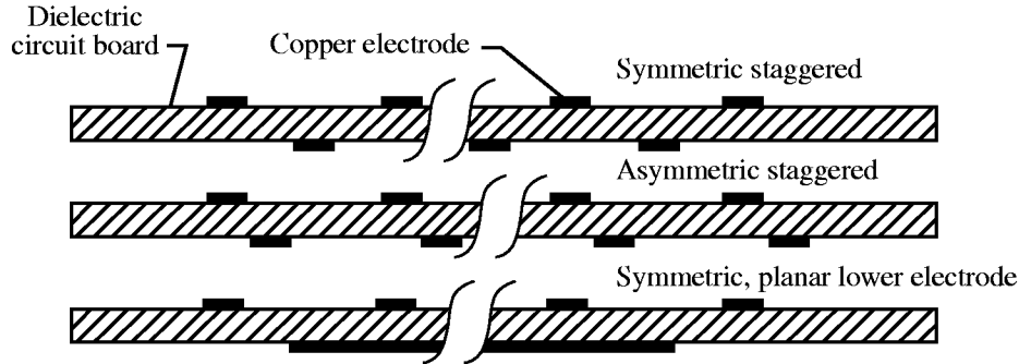
Figure 3.13. Sketch of paraelectric plasma actuator (Roth, Sherman, and Wilkinson 1998).
