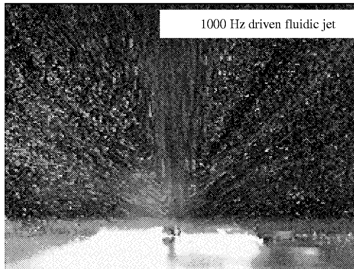
Figure 3.12. Laser-sheet flow visualization of flow field induced by synthetic jet actuator (Joslin, Horta, and Chen 1999).
