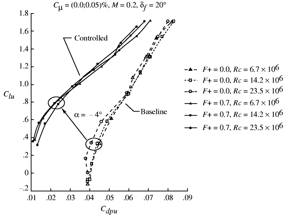
Figure 3.26. Lift-drag polars from separation control experiment (Seifert and Pack 1999b).
