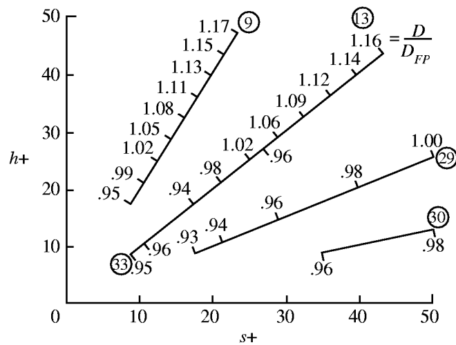
Figure 3.22. Ratio of drag using v-groove riblets to flat plate drag versus height ( h+ ) to spacing ( s+ ) variations (Walsh, 1980).
