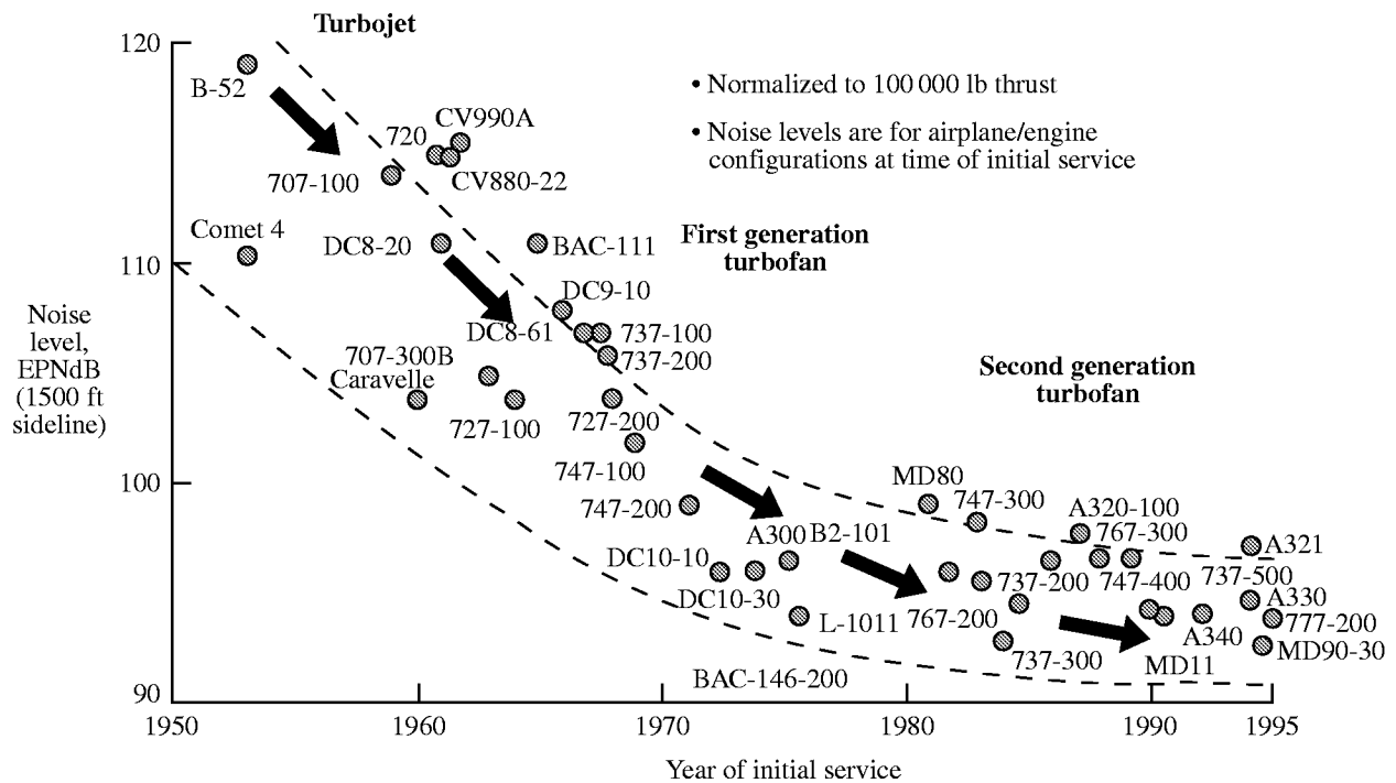
Figure 4.1. History of sideline noise levels at time of aircraft certification (adapted from Condit 1996).
