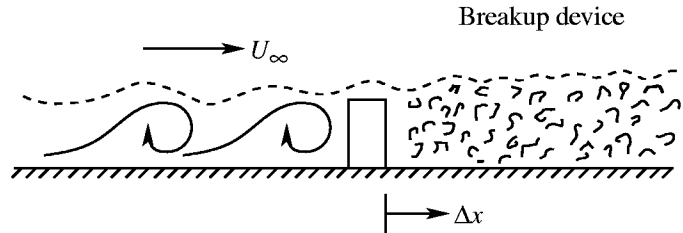
Figure 3.24. Schematic of how an LEBU device affects a turbulent boundary layer (Hefner, Weinstein, and Bushnell 1980).
