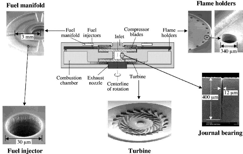
Figure 8.1. MIT microengine assembly and components (from Epstein 2001).
