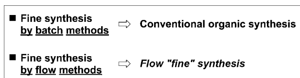
Figure 2. Conventional organic synthesis and flow "fine" synthesis.
