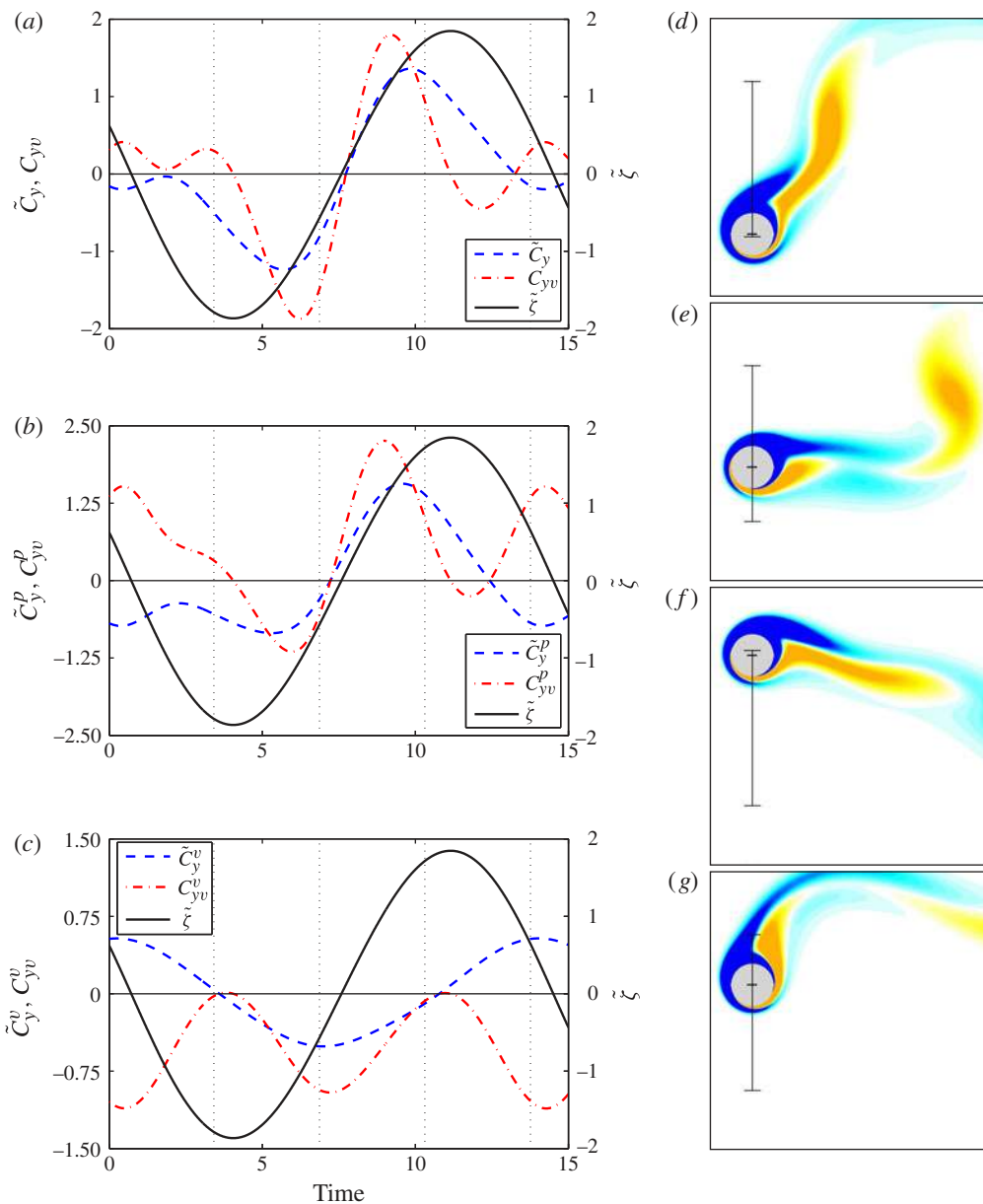
FIGURE 14. (Colour online) Same as figure \Gamma , but now for (\alpha, U^*) = (3.5, 13) – T + S pattern. In panels (d–g), the isocontours of vorticity are in the range \omega_z = \pm 1 .
