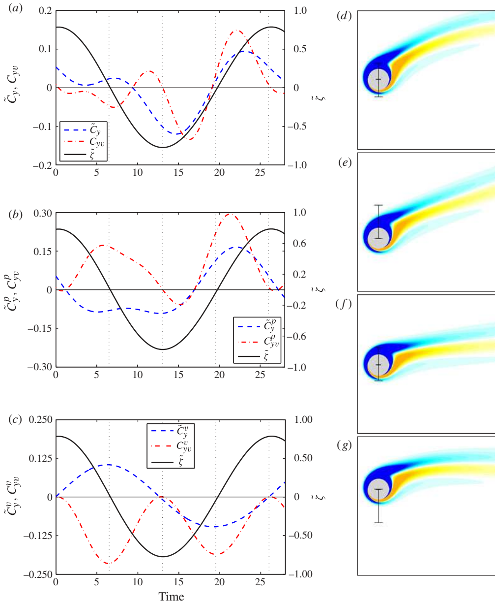
FIGURE 15. (Colour online) Same as figure \square , but now for (\alpha, U^*) = (3, 25) – U pattern. In panels (d–g), the isocontours of vorticity are in the range \omega_z = \pm 1 .
