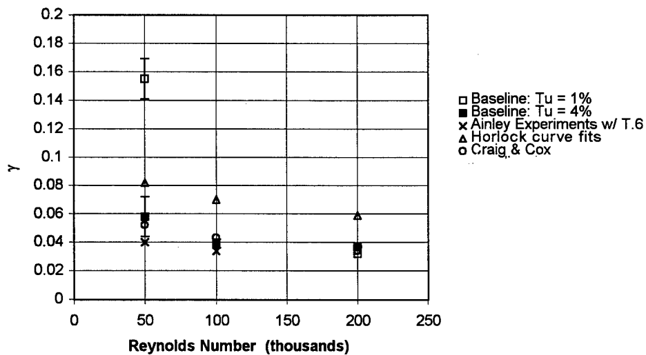
Figure 42. Baseline Pak-B exit loss coefficients.
