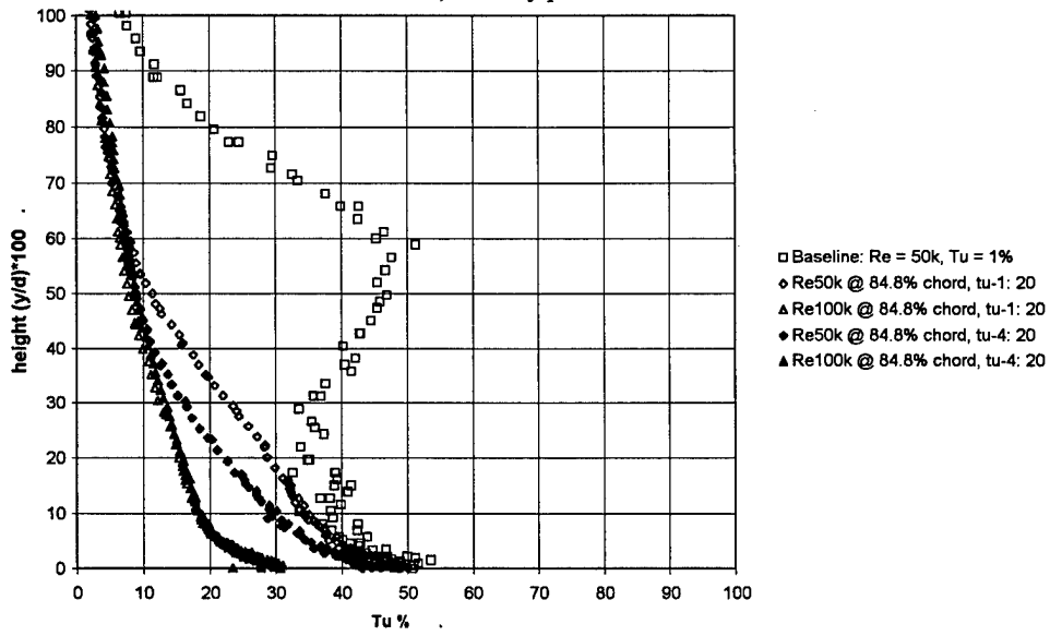
b) local turbulence profile
