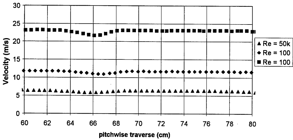
b) Exit velocities for Tu = 4%
