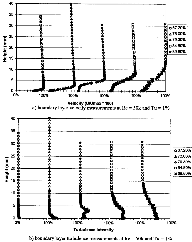
Figure 98. Measured velocity and turbulence profiles between dimples at 50%.
