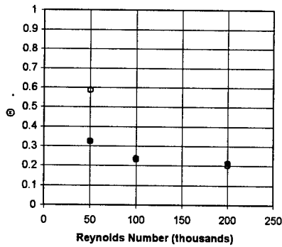
c) Dimples at 55% chord
