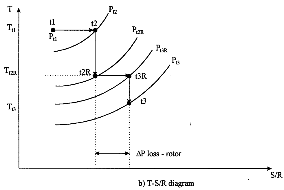
Figure 3. T-S diagram of a typical low pressure turbine stage.
