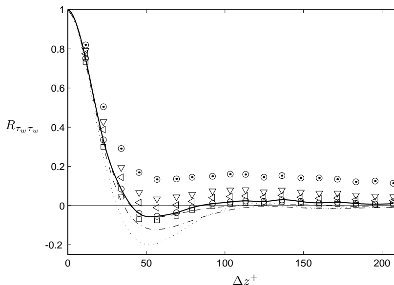
FIGURE 3. Spanwise correlation coefficient R_{\tau_w \tau_w} as a function of \Delta z^+ , Re_\theta = 9500 ( Re_\tau = 2300 ). Present data, \odot : unfiltered, \nabla : f_c^+ = 1.3 \times 10^{-3} , \triangleleft : f_c^+ = 2.6 \times 10^{-3} , \circ : f_c^+ = 5.3 \times 10^{-3} , \square : f_c^+ = 7.9 \times 10^{-3} , —: spline fit to \circ . DNS of channel flow, correlations of u at y^+ = 5 , —: Re_\tau = 590 , - · -: Re_\tau = 395 , · · ·: Re_\tau = 180 (Kim et al. 1987; Moser et al. 1999).
