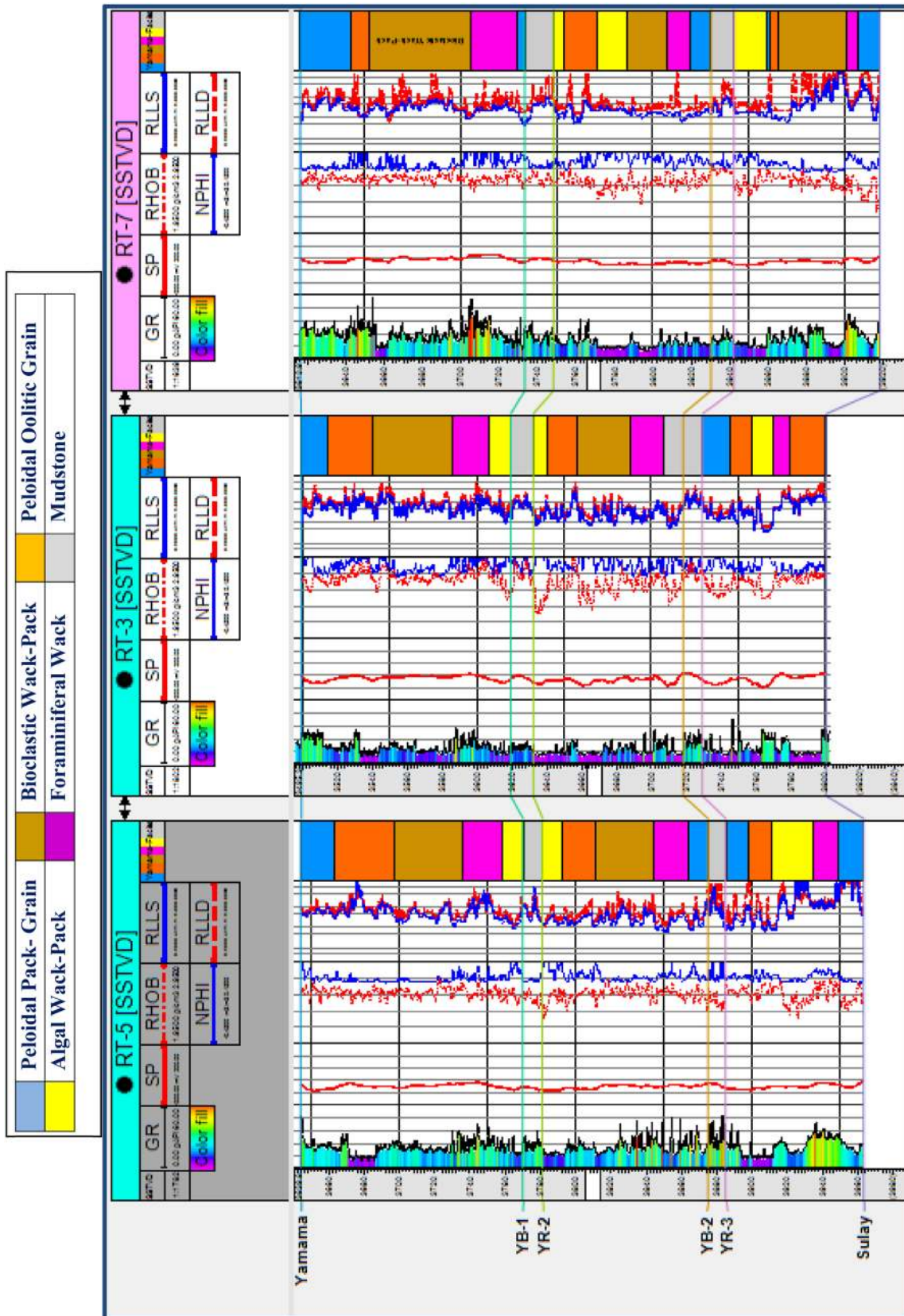
Fig. 3 Cross section for wells Rt-5, 3, and 7 in the Yamama formation
