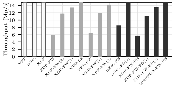
Figure 7: Packet forwarding rates of bare packet I/O engines (white), stateful packet processing w/o FlowBlaze (light gray) and that with FlowBlaze (dark gray): Numbers in ( ) indicate the number of CPU cores if not 1. FlowBlaze does not add overhead (XDP-FW vs XDP-FW-FB) and it scales well (XDP-FW-FB vs XDP-FW-FB(2) and mSw.-FB vs mSw.-FB(2)). The NetFPGA implementation can always forward at line rate while saving up to 3 CPU cores.
