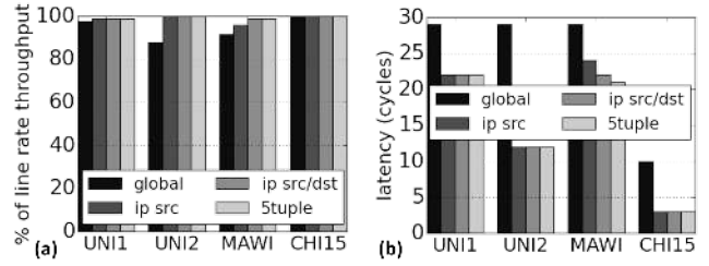
Figure 11: sim1 (a) throughput and (b) latency.
