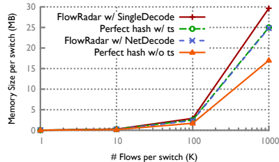
Figure 3: Memory usage per switch
