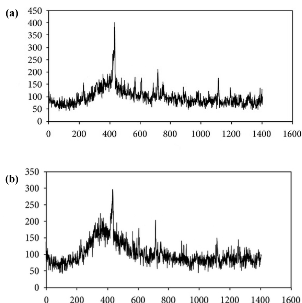
Figure 2. Wide-Angle X-Ray Scattering (WAXS) analysis of malignant human cancer cells and tissues (a) before and (b) after irradiating of synchrotron radiation in transformation process to benign human cancer cells and tissues with the passing of time [1-182]
