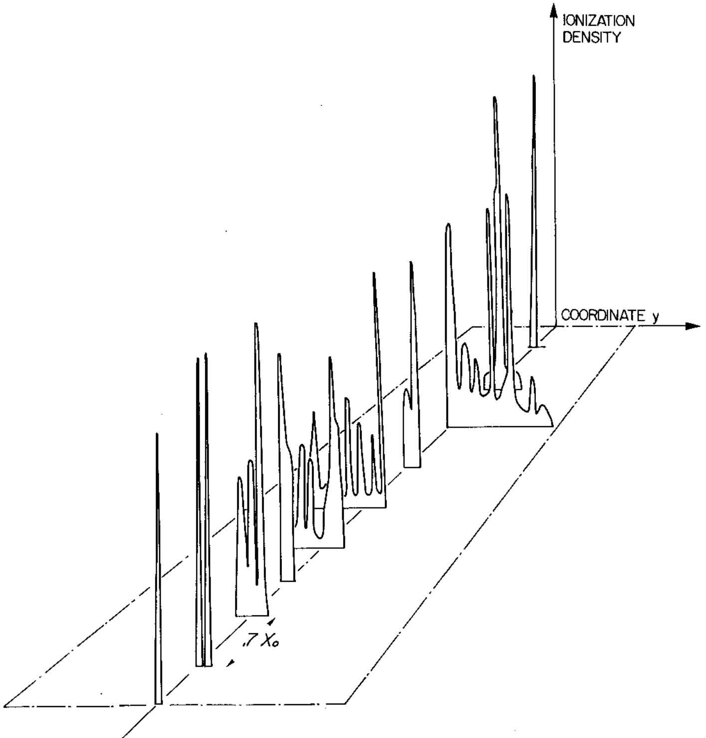
Fig. 10 : Perspective view of the energy depositions in the gas gaps of a quantameter by a Monte Carlo generated 1 GeV electron shower. Note the large fluctuations happening, far from the shower axis, in the third and the fifth active layers.
