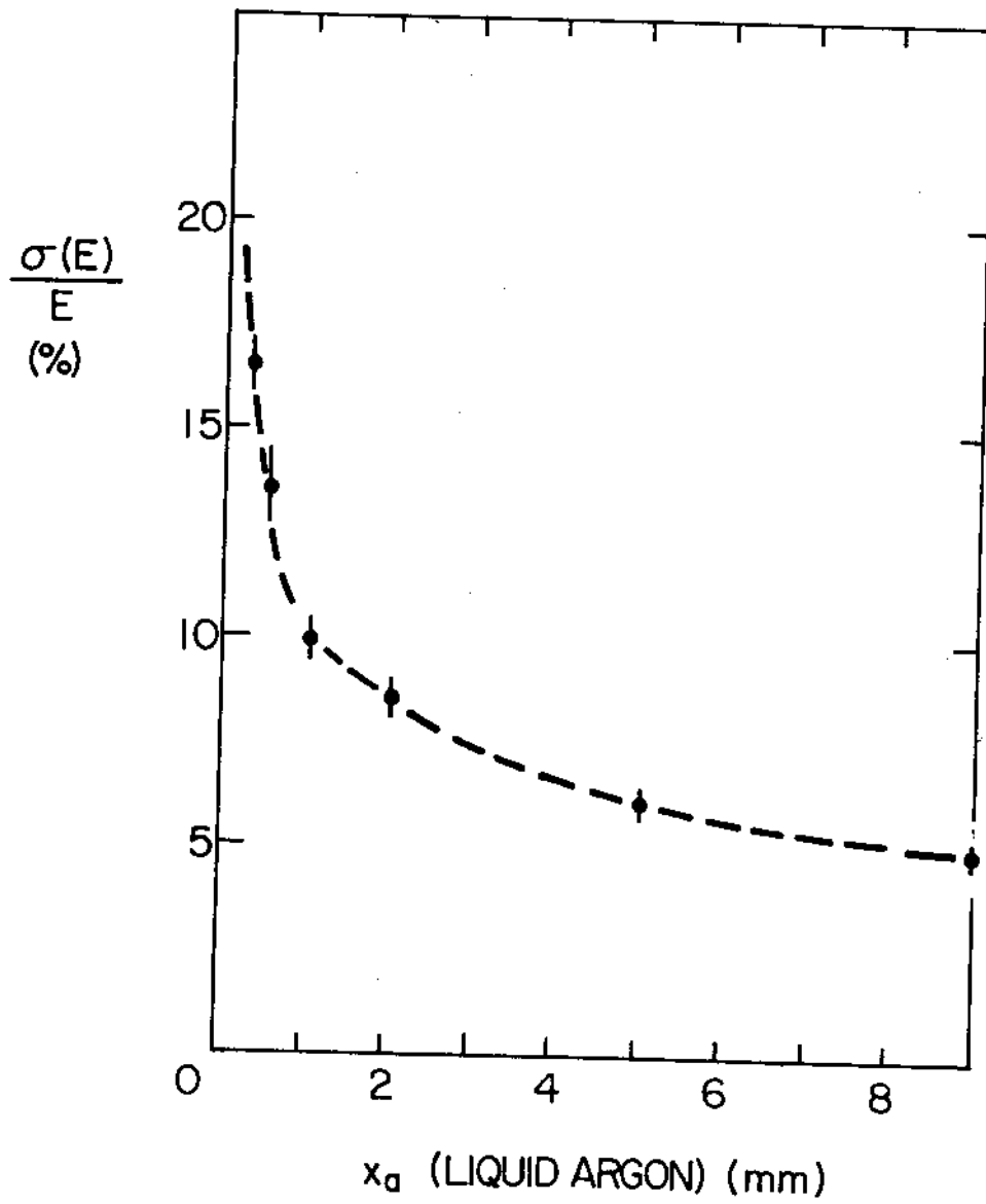
Fig. 9 : Energy resolution versus thickness of the active layers for 1 GeV electrons in an iron-argon calorimeter. 15)
