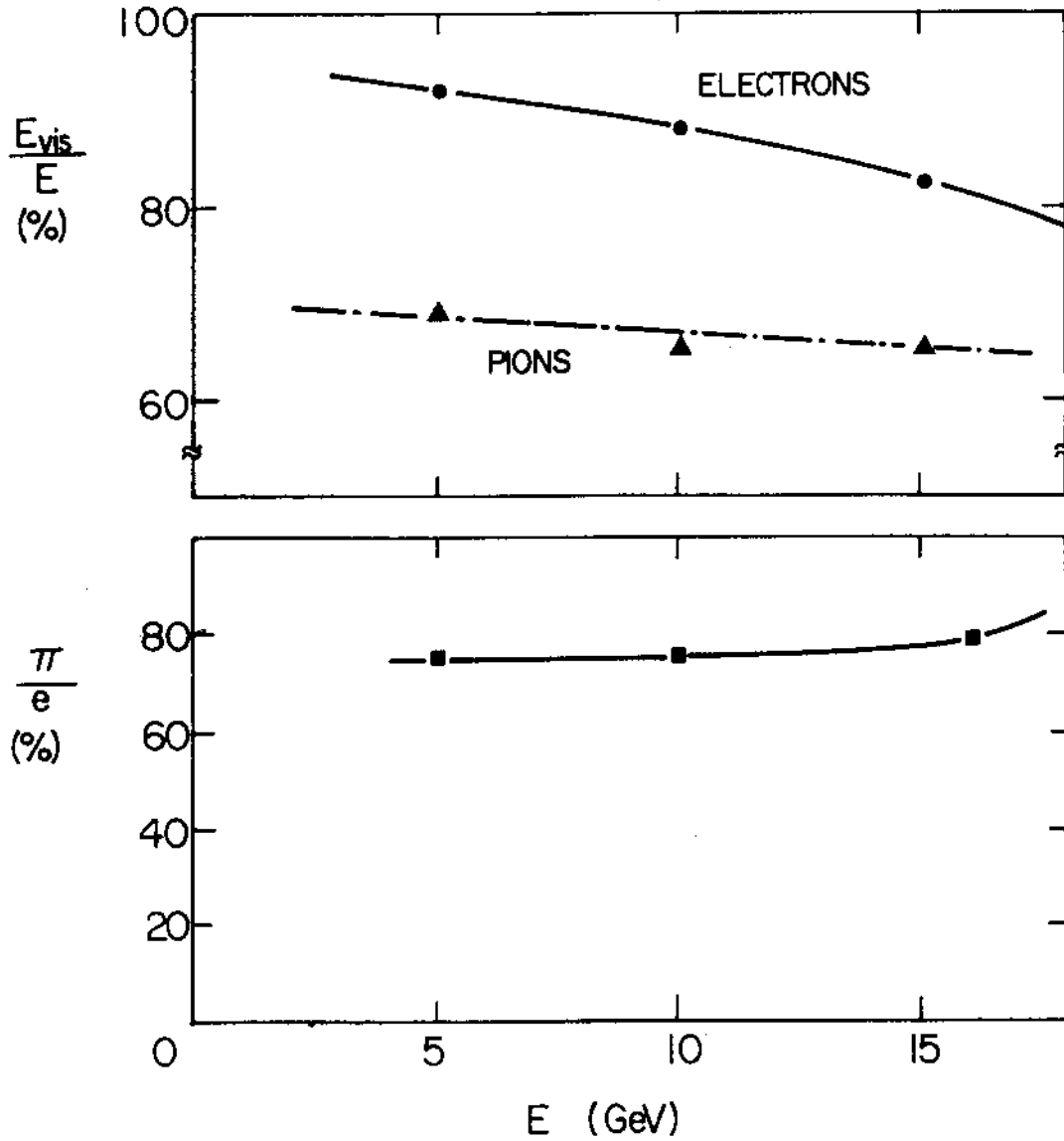
Fig. 13 : Ratio of the visible energy to the incoming energy for electrons and pions illuminating the calorimeter of Cheshire et al. 28)
