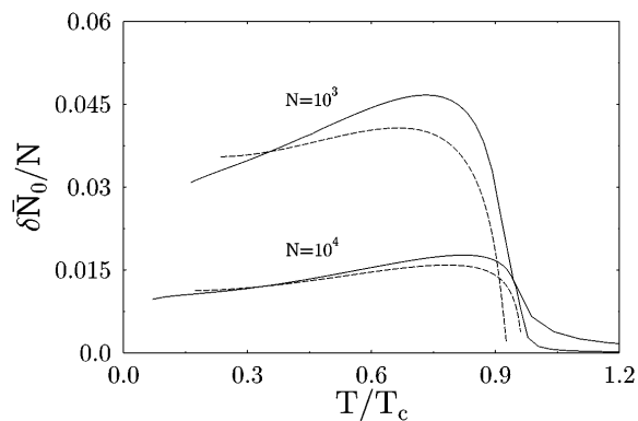
FIG. 2. Relative fluctuations of the ground state occupation number \delta\bar{N}_0/N as a function of the microcanonical temperature for the system of N = 1000 and N = 10000 particles. The full lines represent the numerical results while the dashed lines correspond to the analytic formula. The saddle point method does not allow us to determine fluctuations for very low temperatures.
