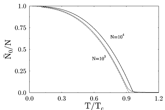
FIG. 1. Relative occupation of the ground state \bar{N}_0/N as a function of the microcanonical temperature for the system of N = 1000 and N = 10000 particles. Full lines represent the numerical results while the dashed lines correspond to the analytic formula. The saddle point method does not allow us to determine the ground state population for very low temperatures.
