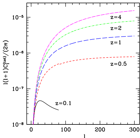
FIG. 10: The total \ell(\ell + 1)C_\ell(z, z)/(2\pi) is shown for z = 4, 2, 1, 0.5 and 0.1 (from top to bottom). Note that for z > 0.1 it reproduces simply C_\ell^{(5)} . For z = 0.1 the contribution of the Doppler part of \ell(\ell + 1)C_\ell^{(3)}(z, z)/(2\pi) is important, which we have computed only for \ell \lesssim 80 . For clarity, we have again chosen a log representation in this graph.
