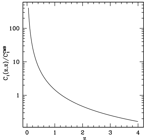
FIG. 3: We show the dipole amplitude in units of the CMB dipole as a function of z = z' in a pure CDM universe.
