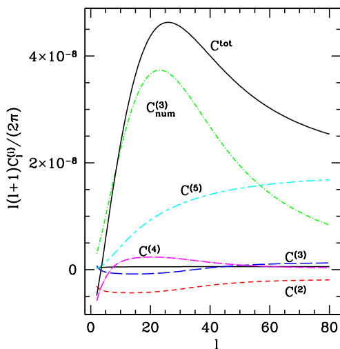
FIG. 11: The different contributions to \ell(\ell + 1)C_\ell(z, z)/(2\pi) for z = 0.1 are shown. For this low redshift they are all of the same order of magnitude. For low \ell 's our approximations are not trustable, they even lead to negative values for C_\ell^{tot} for \ell \leq 3 .
