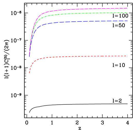
FIG. 12: The contribution \ell(\ell + 1)C_\ell^{(5)}(z, z')/(2\pi) is shown as a function of z with z' fixed to z' = 0.5 and \ell = 200, 100, 50, 10 and 2 (from top to bottom). Above \ell \simeq 50 , the \ell -dependence of the result becomes weak as expected. For z > 0.1 this represents actually also the total contribution to C_\ell .
