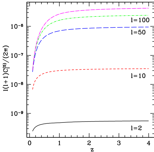
FIG. 13: Like Fig. 12, but for z' = 1 .
