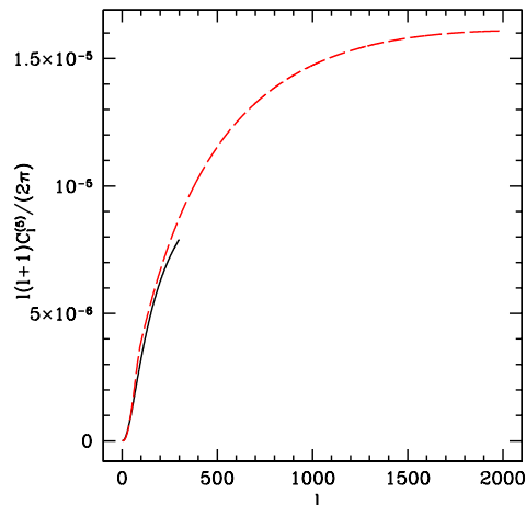
FIG. 15: The approximation for \ell(\ell + 1)C_\ell^{(5)}(z, z')/(2\pi) given in Eq. (E15) (red, dashed line) is compared with our numerical result (black, solid line) for z = 2 .
