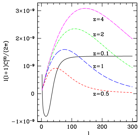
FIG. 6: The contribution \ell(\ell+1)C_\ell^{(3)}(z,z)/(2\pi) , without the numerical part, for z = 4, 2, 1, 0.5 and 0.1 (from top to bottom). Note that here we have chosen linear as opposed to a log representation.
