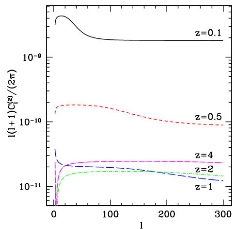
FIG. 5: The contribution C_\ell^{(2)} . We choose the same colors (linestyles) like in Fig. 4. The contributions for z = 0.1, 0.5 and 1 are negative while those for z = 2, 4 pass through 0 at low \ell , visible as a spike. This may well be due to our approximative treatment.
