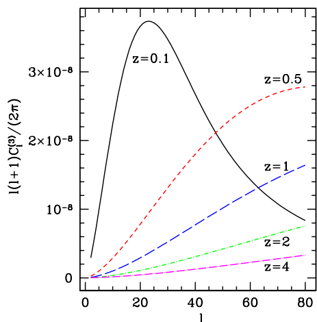
FIG. 7: The Doppler contribution of \ell(\ell+1)C_\ell^{(3)}(z,z)/(2\pi) which has been determined numerically for z = 0.1, 0.5, 1, 2 and 4 (from top to bottom). Our numerical code is stable only for \ell \lesssim 80 and we therefore plot only this part of the curve.
