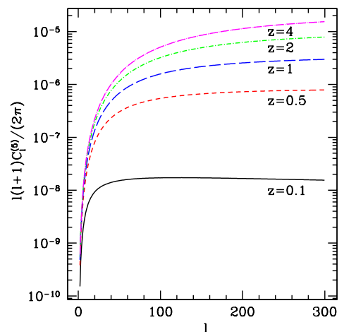
FIG. 9: The lensing contribution \ell(\ell+1)C_\ell^{(5)}(z,z)/(2\pi) for z = 4, 2, 1, 0.5 and 0.1 (from top to bottom). For clarity, we have again chosen a log representation in this graph.
