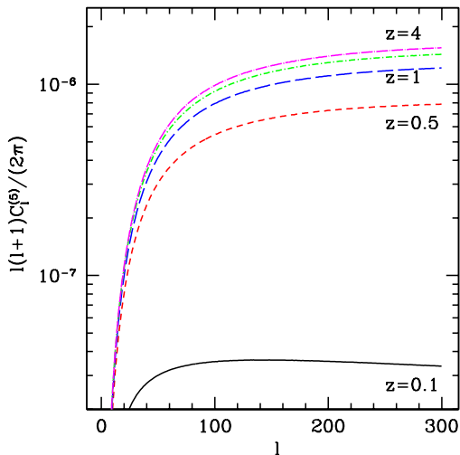
FIG. 14: The contribution \ell(\ell + 1)C_\ell^{(5)}(z, z')/(2\pi) is shown for z' = 0.5 and z = 4, 2, 1, 0.5 and 0.1 (from top to bottom). Again, for z \neq 0.1 this result is equivalent to the full C_\ell .
