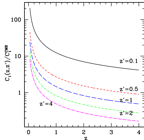
FIG. 2: We show the dipole amplitude in a pure CDM universe in units of the CMB dipole as a function of z for z' = 0.1, 0.5, 1, 2 and 4 from top to bottom.
