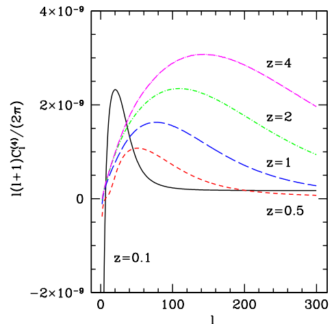
FIG. 8: The contribution \ell(\ell+1)C_\ell^{(4)}(z,z)/(2\pi) for z = 4, 2, 1, 0.5 and 0.1 (from top to bottom).
