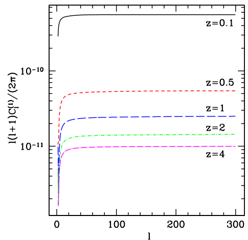
FIG. 4: The contribution of the redshift term \ell(\ell + 1)C_\ell^{(1)}(z, z)/(2\pi) for z = 0.1, 0.5, 1, 2 and 4 (from top to bottom).
