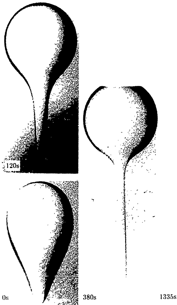
Fig. 5. - (After Koh&Leal [1990] © American Institute of Physics). Unstable spherical drop of 10,000 cS Dow silicone oil ( \mu = 101 \text{ P} , \rho = 0.972 \text{ gm/cm}^3 ) in Pale 1,000 oil (oxidized castor oil, \mu = 391 \text{ P} , \rho = 1.021 )
