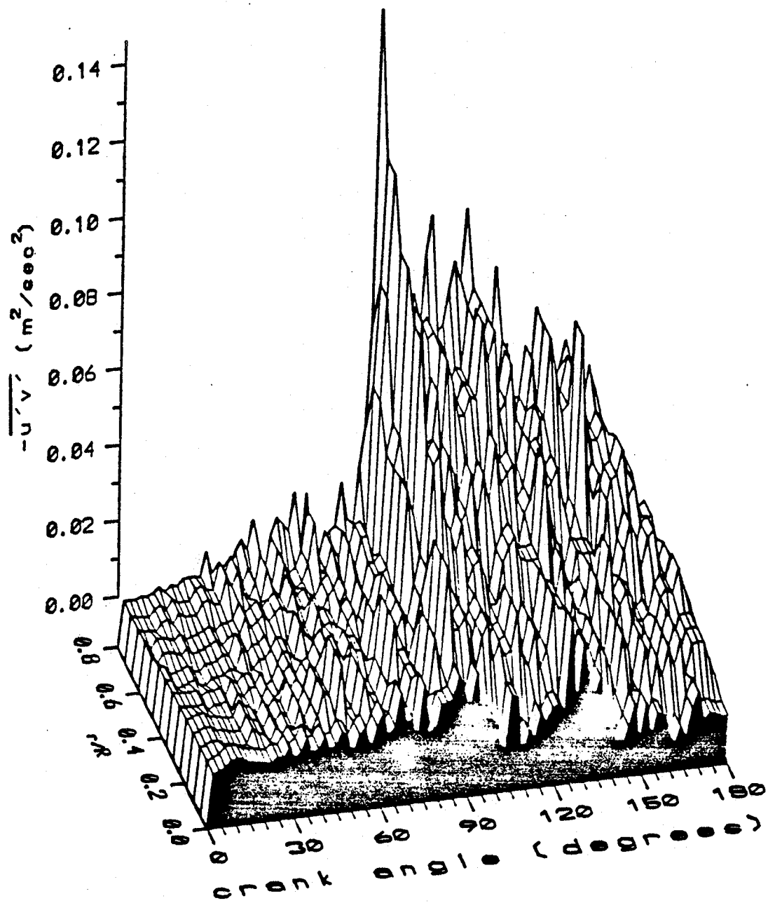
Figure 22: Reynolds shear stress at s/d = 30 (not smoothed)
