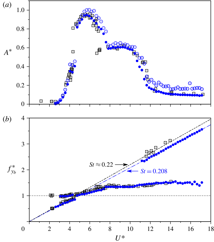
FIGURE 3. (Colour online) A comparison of experimental results shows excellent agreement between the present study and Khalak & Williamson (□) in (a) the amplitude and (b) the frequency responses of a circular cylinder with m^* = 2.4 . In (a) open circles represent the normalized amplitude peaks, A_{max}^* , of the present results, solid circles represent the present A_{10}^* values, the mean of the top 10% of the oscillation amplitudes, and open squares represent the results of Khalak & Williamson (□). In (b) solid circles represent the present results, while open squares represent the results of Khalak & Williamson (□).
