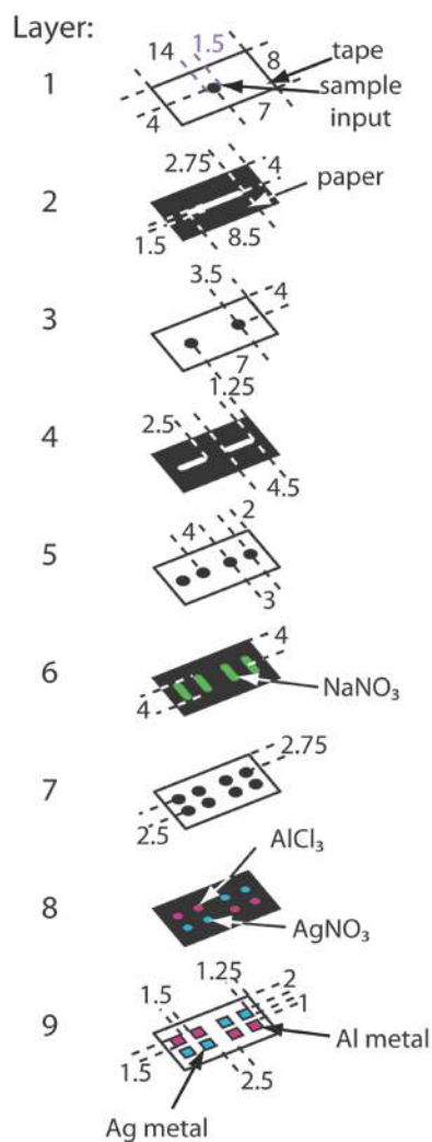
Figure S3. Expanded view of a 4-cell battery. All values shown are in millimeters. The device is 14-mm wide × 8-mm long.
