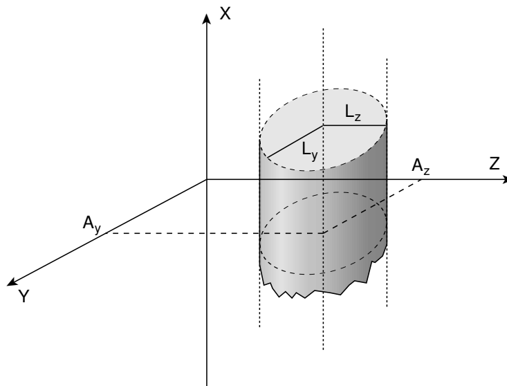
Fig. 8.13: Infinite Elliptical Cylinder parallel to the x-axis (XEC)
