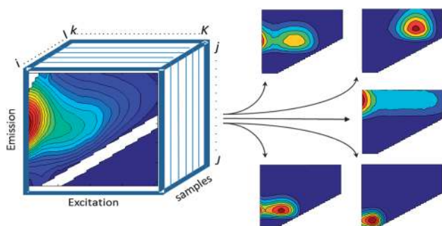
Fig. 2 EEM dataset arranged in a threeway structure and decomposed into five PARAFAC components.
