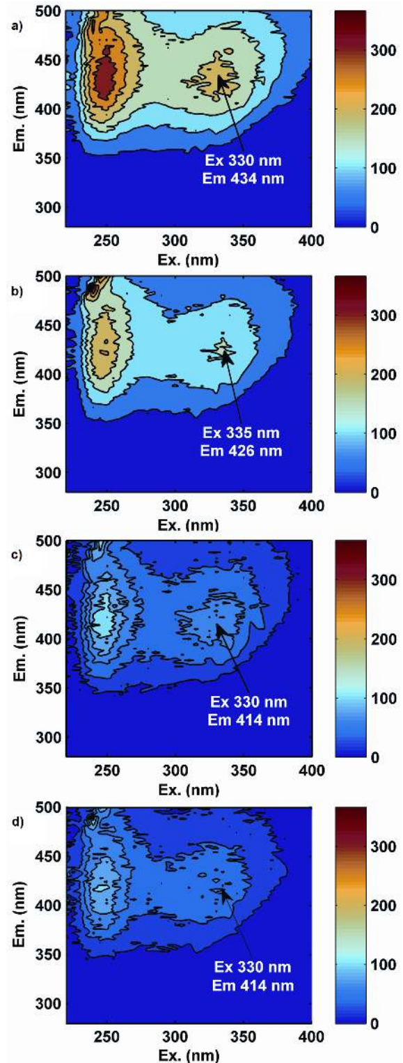
Figure 2. Fluorescence EEMs of raw (a), post-clarification (b), post-GAC (c), and final water (d) at site 13 collected on 5 August 2007. The location of peak C fluorescence maximum indicated with arrow. Fluorescence emission intensity in arbitrary units.
