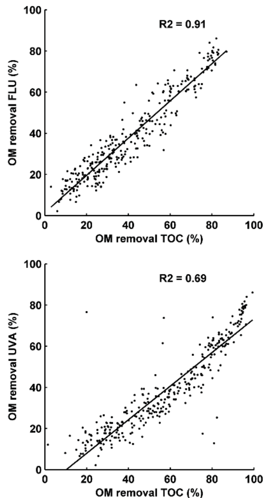
Figure 4. OM removal prediction with differential fluorescence (OM removal FLU) and differential UVA (OM removal UVA) between raw and clarified water.
