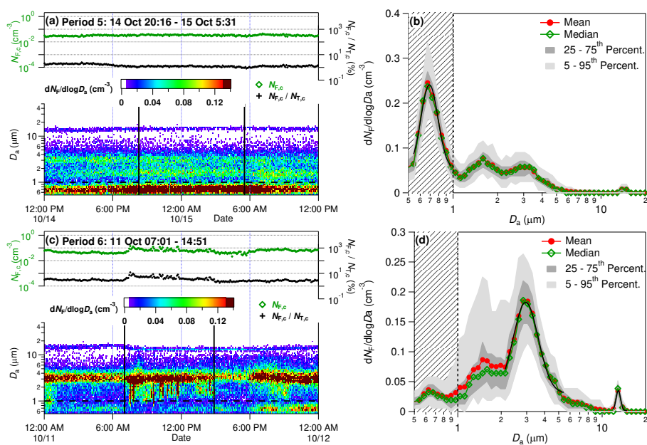
Fig. 9. Characteristic FBAP number size distribution patterns observed during exemplary periods #5 and #6 (plots analogous to Fig. 7). (a)–(b) Period #5; Fit 5.1: D_a=0.54\text{--}0.96 \mu\text{m} ; D_{a,g}=0.74 \mu\text{m} , \sigma_g=1.14 , N=2.7 \times 10^{-1} \text{cm}^{-3} ; (c)–(d) Period #6; Fit 6.1: D_a=2.1\text{--}5.4 \mu\text{m} ; D_{a,g}=3.0 \mu\text{m} , \sigma_g=1.22 , N=3.3 \times 10^{-2} \text{cm}^{-3} ; Fit 6.2: D_a=12.0\text{--}14.9 \mu\text{m} ; D_{a,g}=13.0 \mu\text{m} , \sigma_g=1.04 , N=1.30 \times 10^{-3} \text{cm}^{-3} .
