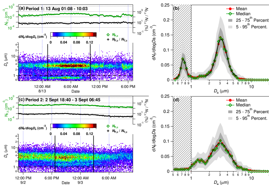
Fig. 7. Characteristic FBAP number size distribution patterns observed during exemplary periods #1 and #2. Left panels show time series of N_{F,c} , N_{F,c}/N_{T,c} ratio and dN_F/d\log D_a on days of interest (analogous to Fig. 1), and black vertical lines indicate time periods over which exemplary size distributions were averaged ( dN_F/d\log D_a vs. D_a , right panels). Red traces represent mean values, green traces represent median values, dark gray regions show 25–75th percentile range, and light gray regions show 5–95th percentile range. Hatched area below 1.0 \mu\text{m} indicates particle size range where fluorescent particles were not considered FBAP due to interference with non-biological aerosol. Black traces are lognormal fits to individual peaks (mean values) with the following fit parameters: (a)–(b) Period #1; Fit 1.1: D_a=0.54\text{--}0.90\ \mu\text{m} , D_{a,g}=0.74\ \mu\text{m} , \sigma_g=1.10 , N=6.5\times 10^{-3}\ \text{cm}^{-3} ; Fit 1.2: D_a=1.7\text{--}5.8\ \mu\text{m} ; D_{a,g}=3.2\ \mu\text{m} , \sigma_g=1.22 , N=2.7\times 10^{-2}\ \text{cm}^{-3} ; (c)–(d) Period #2; Fit 2.1: D_a=1.8\text{--}5.8\ \mu\text{m} ; D_{a,g}=3.0\ \mu\text{m} , \sigma_g=1.43 , N=3.7\times 10^{-2}\ \text{cm}^{-3} .
