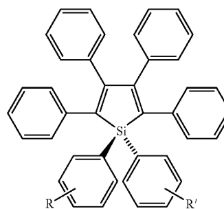
Silole
