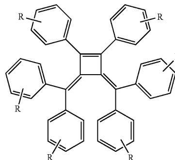
Cyclobutene
