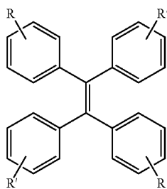
Tetraphenylethylene
