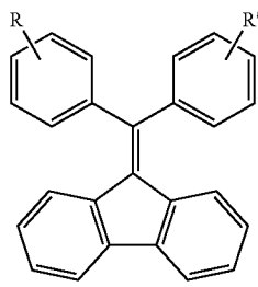
Fulvene
