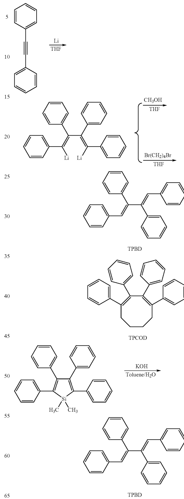
Scheme 4. Synthesis of Butadiene and Cyclobutadiene Derivatives
