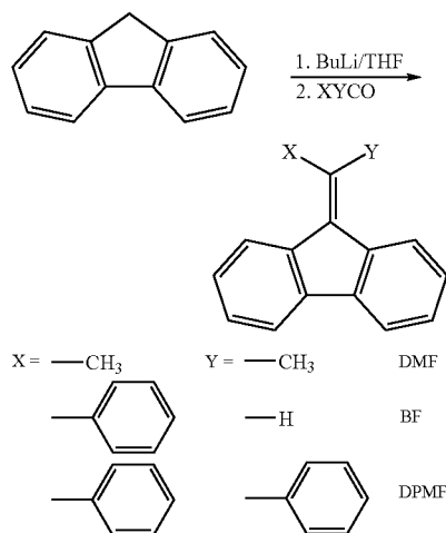
Scheme 5. Synthesis of Fulvene Derivatives
