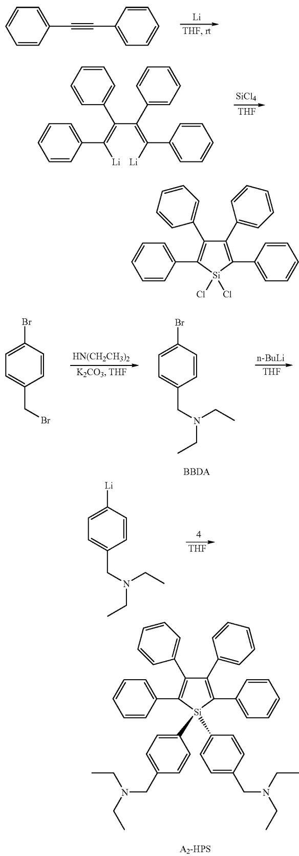
Scheme 3. Synthesis of silole derivatives.
