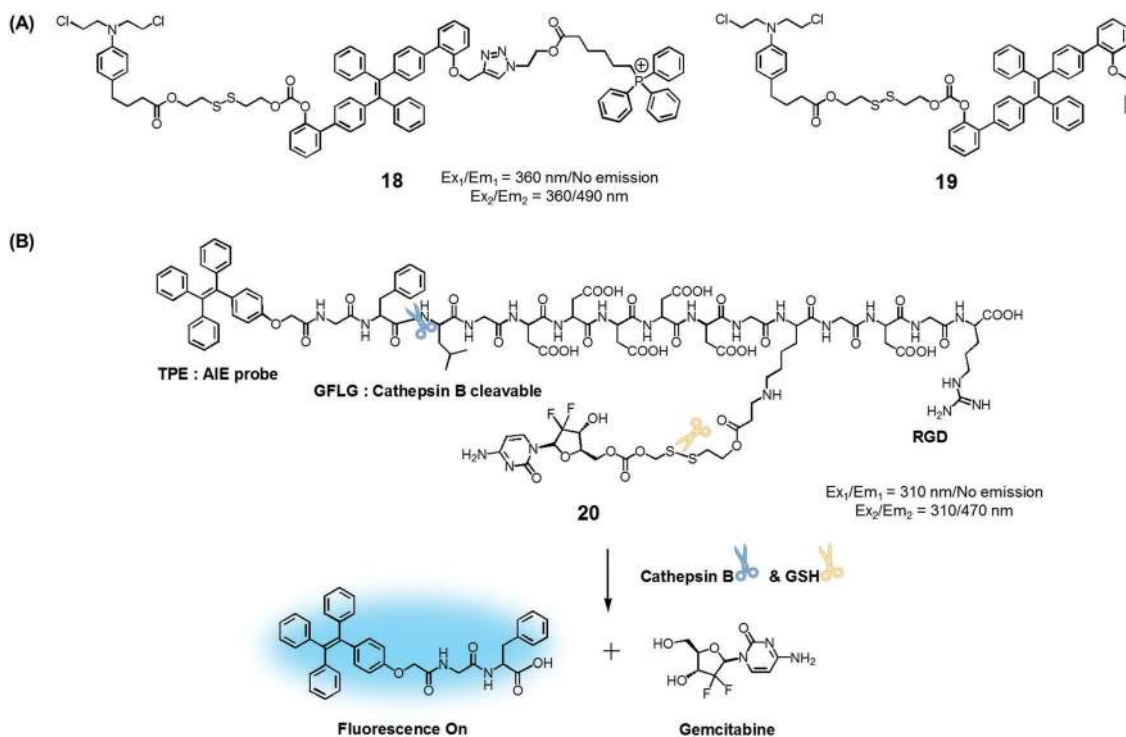
Fig. 8 (A) Thiol-activatable AIE-based theranostic agents 18 and 19 . (B) Conjugate 20 and its activation by GSH and cathepsin B, respectively.
