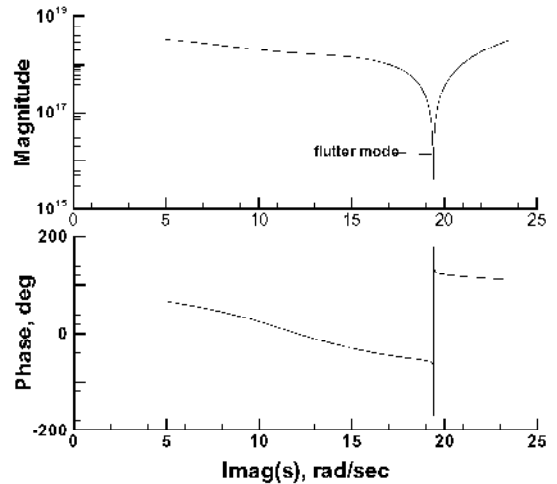
Figure 12. Determinant of stability matrix versus \text{Imag}(s) : transport (BAII) wing model, U = 1056 ft/sec.
