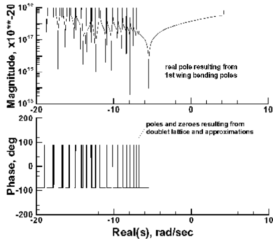
Figure 13. Determinant of stability matrix versus \text{Real}(s) : transport (BAII) wing model, U = 1450 ft/sec.
