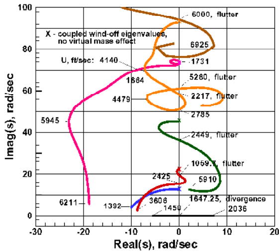
Figure 11. 'Exact' root loci as a function of airspeed showing flutter and divergence: transport (BAII) wing model, M = 0 .
