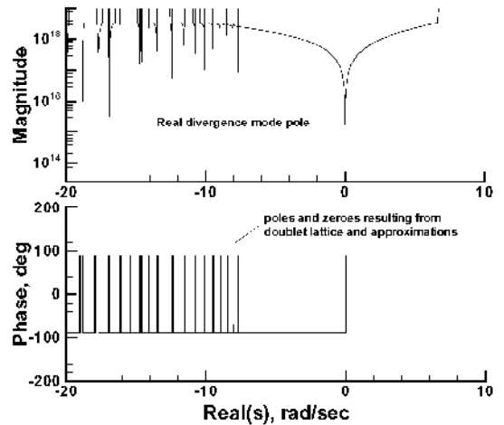
Figure 14. Determinant of stability matrix versus \text{Real}(s) : transport (BAII) wing model, U = 1647.25 ft/sec.
