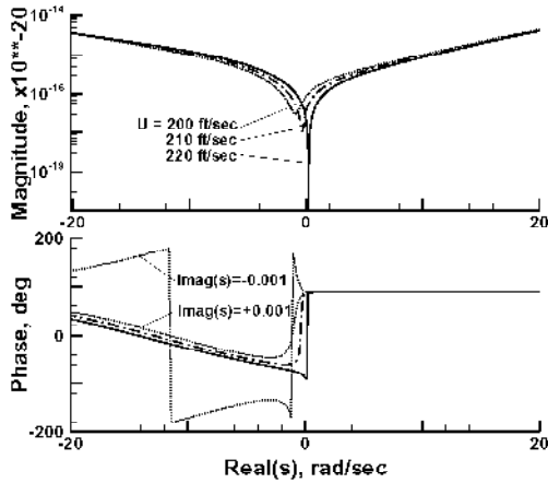
Figure 7. Determinant of stability matrix versus Real(s): two degree of freedom airfoil, c.g. at 45% chord.
